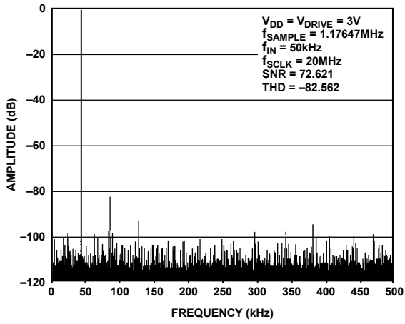
Figure 3. Typical FFT
