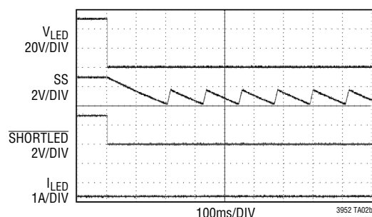
Short LED Protection without R_{SS} : Hiccup Mode
