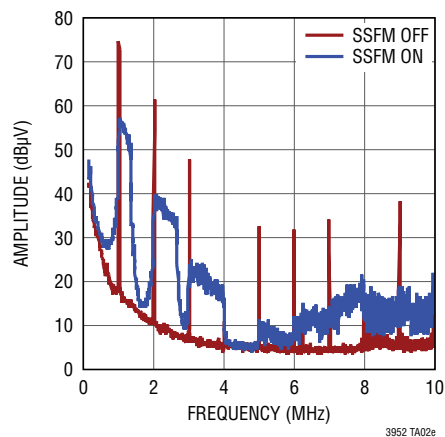
Average Conducted EMI Comparison
