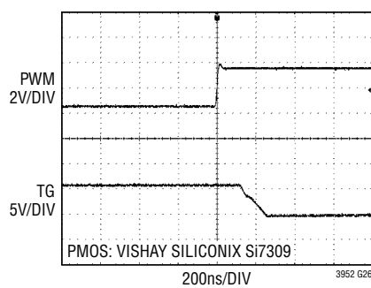
TG Driver Turn-On
