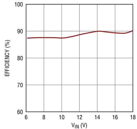
Efficiency Over Working Range
