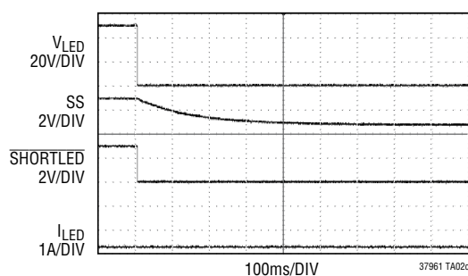
Short LED Protection with R_{SS} : Latchoff Mode
