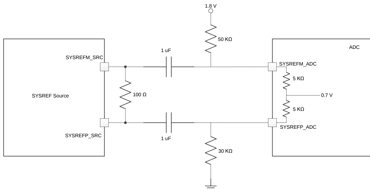
Figure 82. AC-Coupling Scheme for SYSREF (do not use for SYNC~)
