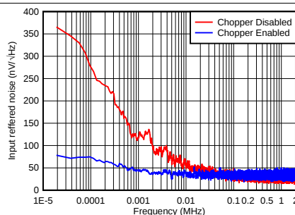
Figure 39. Low-Frequency Noise With and Without Chopper Enabled
