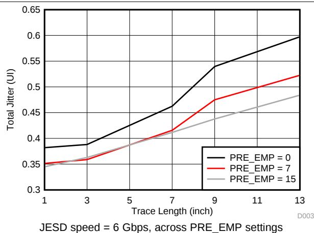
Figure 42. Total Jitter vs Trace Length
