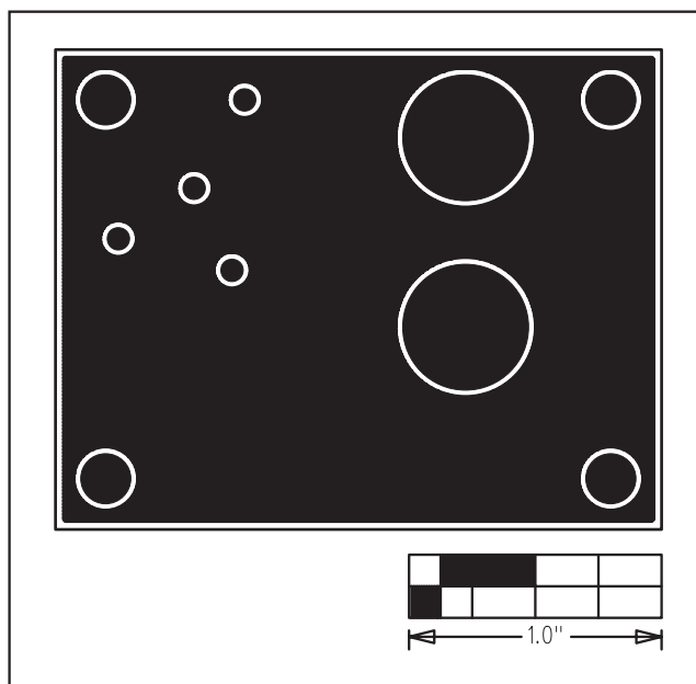
Figure 4. MAX4173 EV Kit PCB Layout—Solder Side
