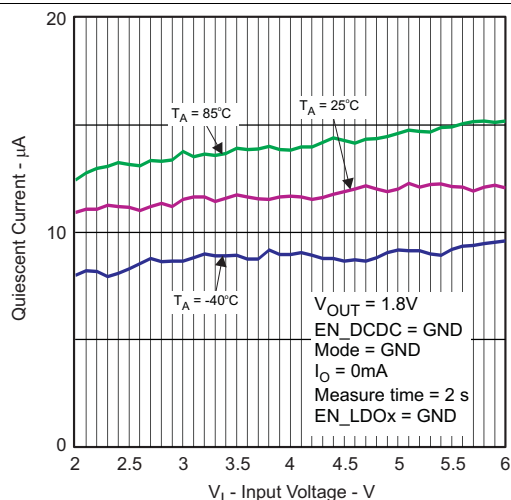
Figure 11. TPS650001 Shutdown Current vs Input Voltage
