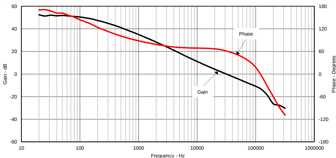
Figure 6. TPS54335AEVM-010 Loop Response
