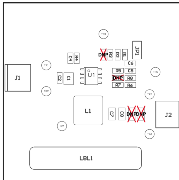
Figure 15. TPS54335AEVM-010 Top-Side Assembly
