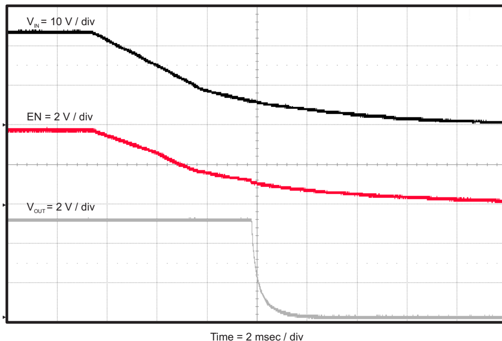
Figure 13. TPS54335AEVM-010 Shut-down Relative to V_{IN}
