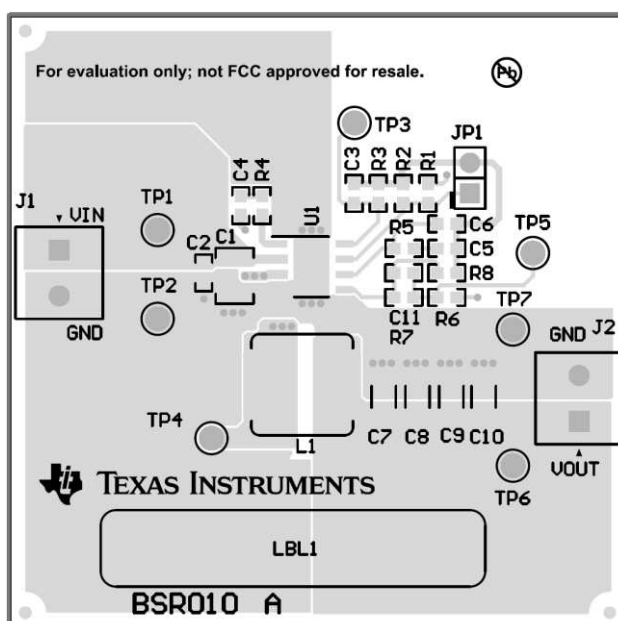
Figure 16. TPS54335AEVM-010 Top-Side Layout
