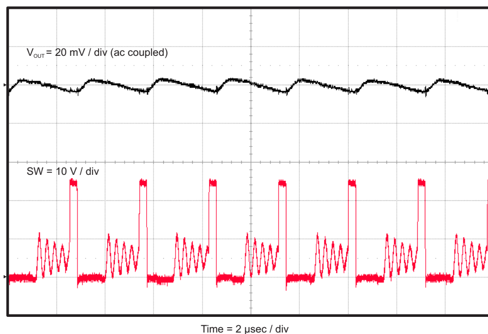
Figure 8. TPS54335AEVM-010 Output Ripple, I_{OUT} = 100 mA
