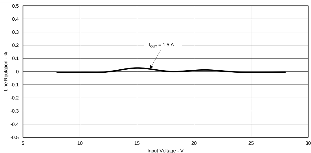
Figure 4. TPS54335AEVM-010 Line Regulation
