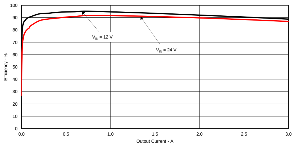
Figure 1. TPS54335AEVM-010 Efficiency
