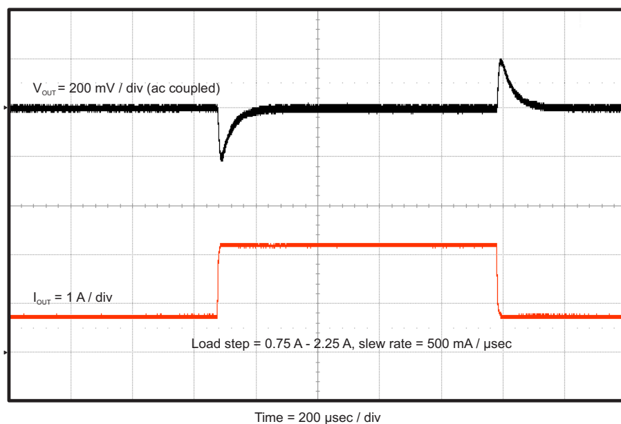
Figure 5. TPS54335AEVM-010 Transient Response
