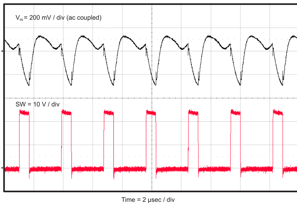
Figure 10. TPS54335AEVM-010 Input Ripple
