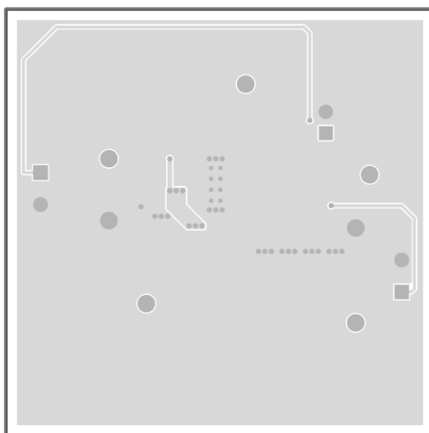
Figure 17. TPS54335AEVM-010 Bottom-Side Layout
