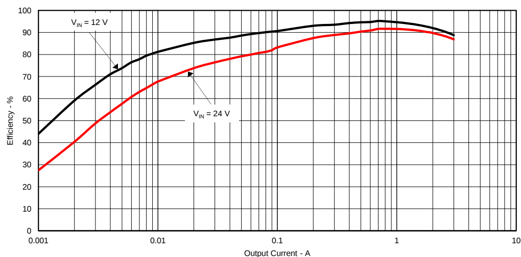
Figure 2. TPS54335AEVM-010 Low Current Efficiency
