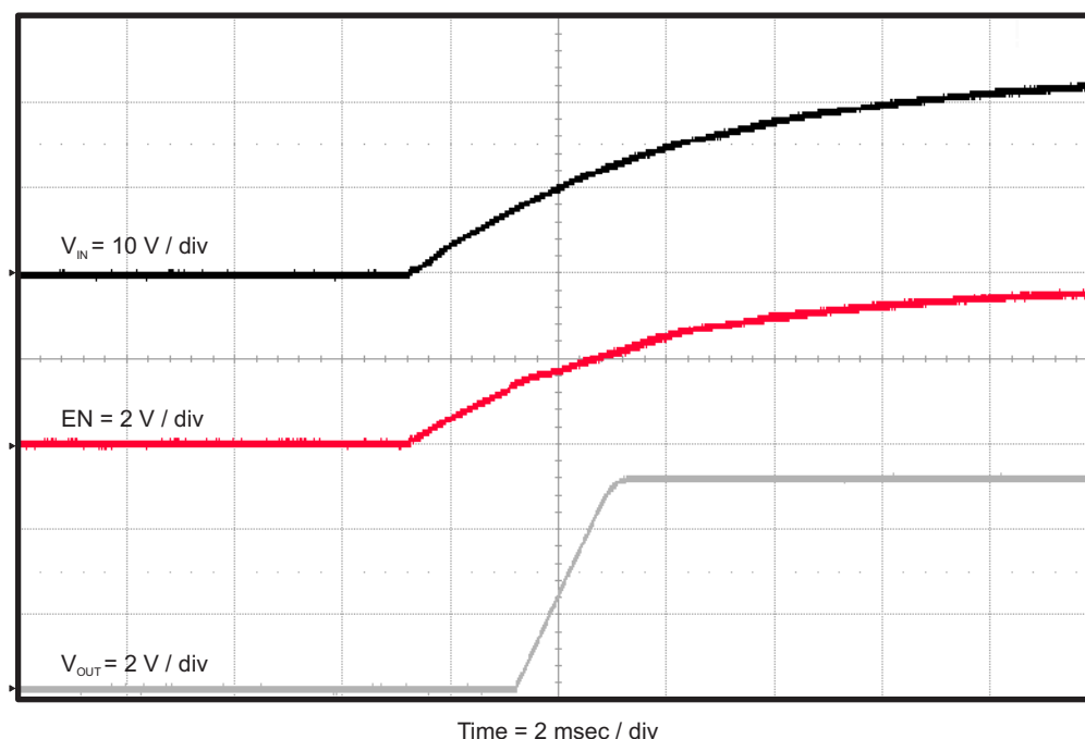
Figure 11. TPS54335AEVM-010 Start-Up Relative to V_{IN}
