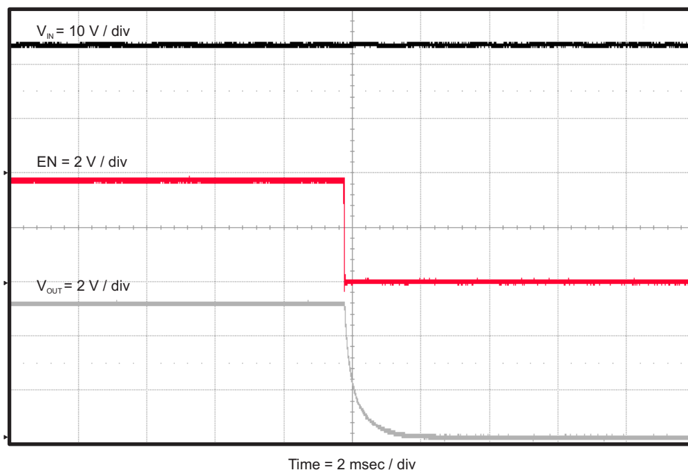
Figure 14. TPS54335AEVM-010 Shut-down Relative to EN
