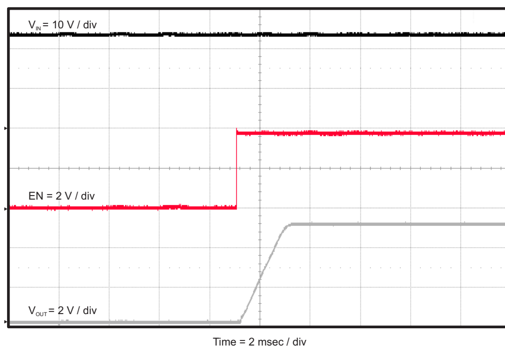
Figure 12. TPS54335AEVM-010 Start-up Relative to Enable
