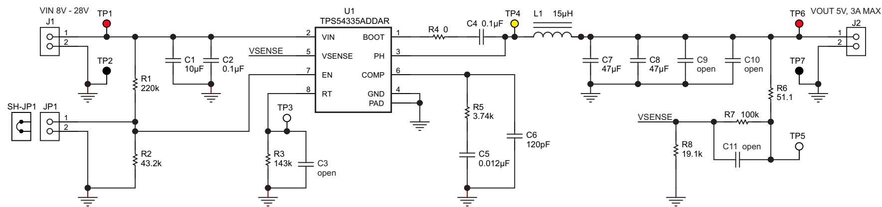
Figure 18. TPS54335AEVM-010 Schematic
