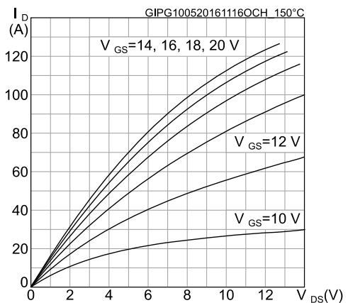
Figure 5: Output characteristics ( T_J = 150\text{ °C} )
