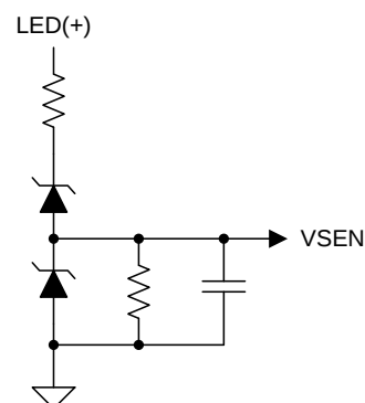
Figure 15. Voltage Sense for Buck-Boost Applications
