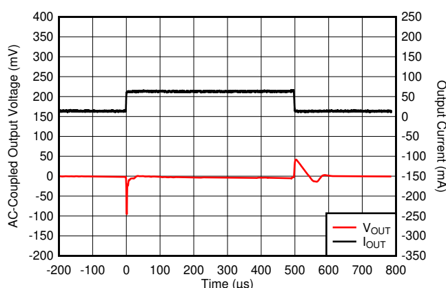
Load Transient Response (V_{IN} = V_{OUT} + 1\text{ V}, C_{OUT} = 1\text{ }\mu\text{F}, I_{OUT} = 1\text{ mA to }50\text{ mA in }1\text{ }\mu\text{s})
