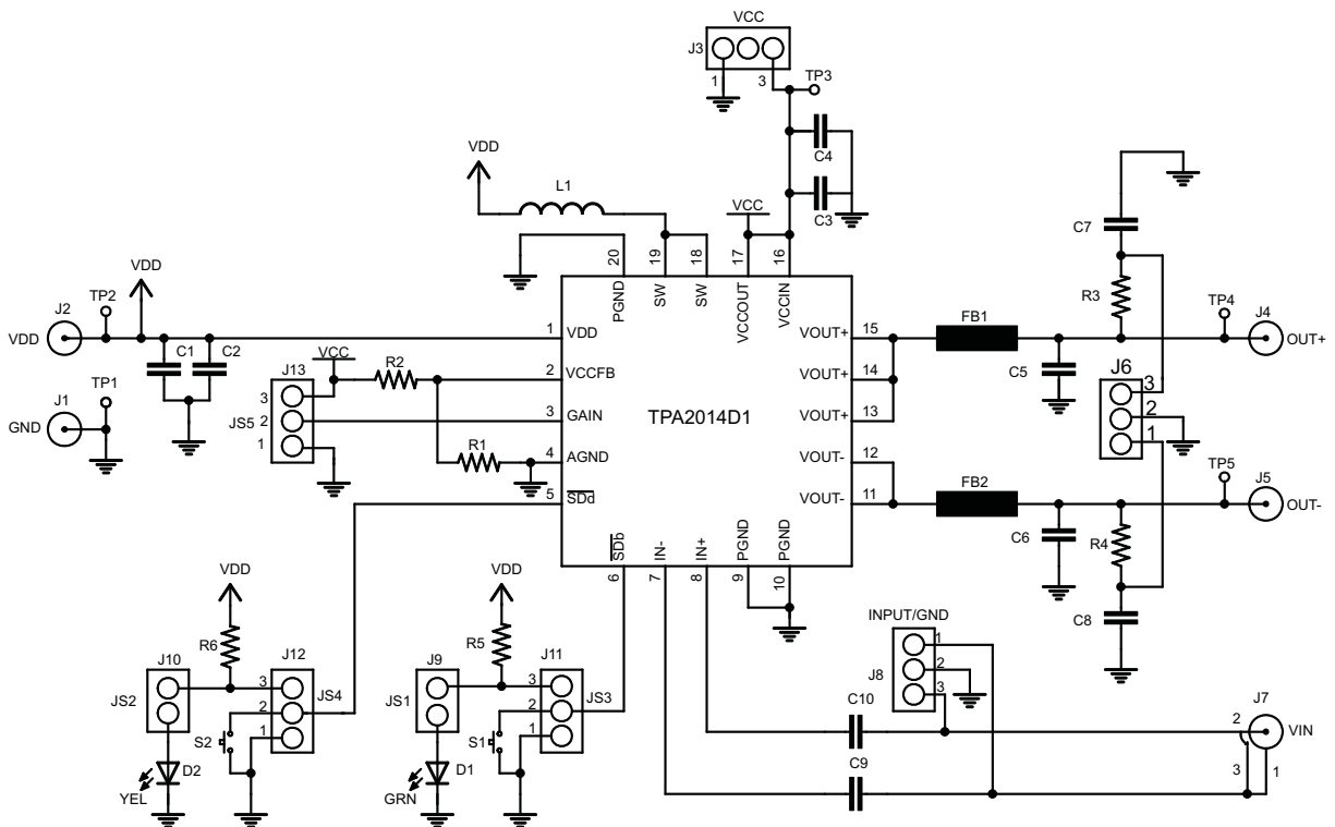
Figure 1. TPA2014D1EVM Schematic
