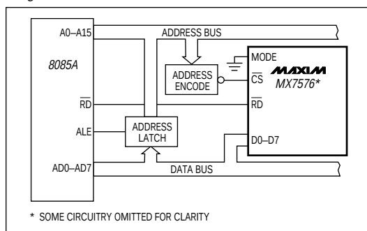
Figure 10. MX7575 to 8085A Asynchronous Conversion Mode Interface
