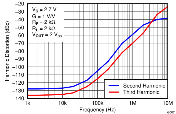
Figure 8. Harmonic Distortion vs Frequency
