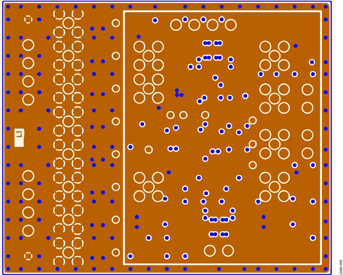
Figure 9. EVAL-ADG5249FEBZ Layer 3
