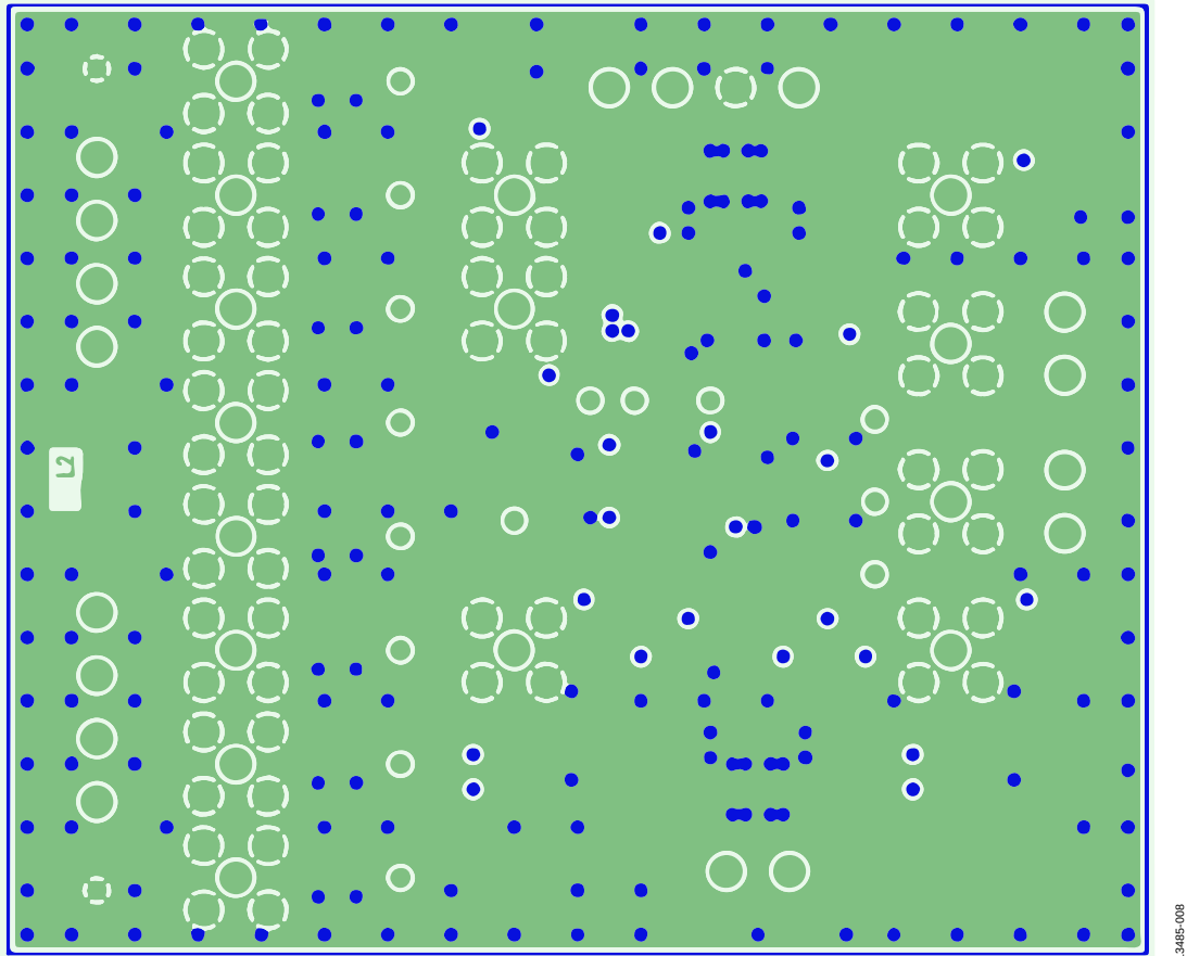
Figure 8. EVAL-ADG5249FEBZ Layer 2
