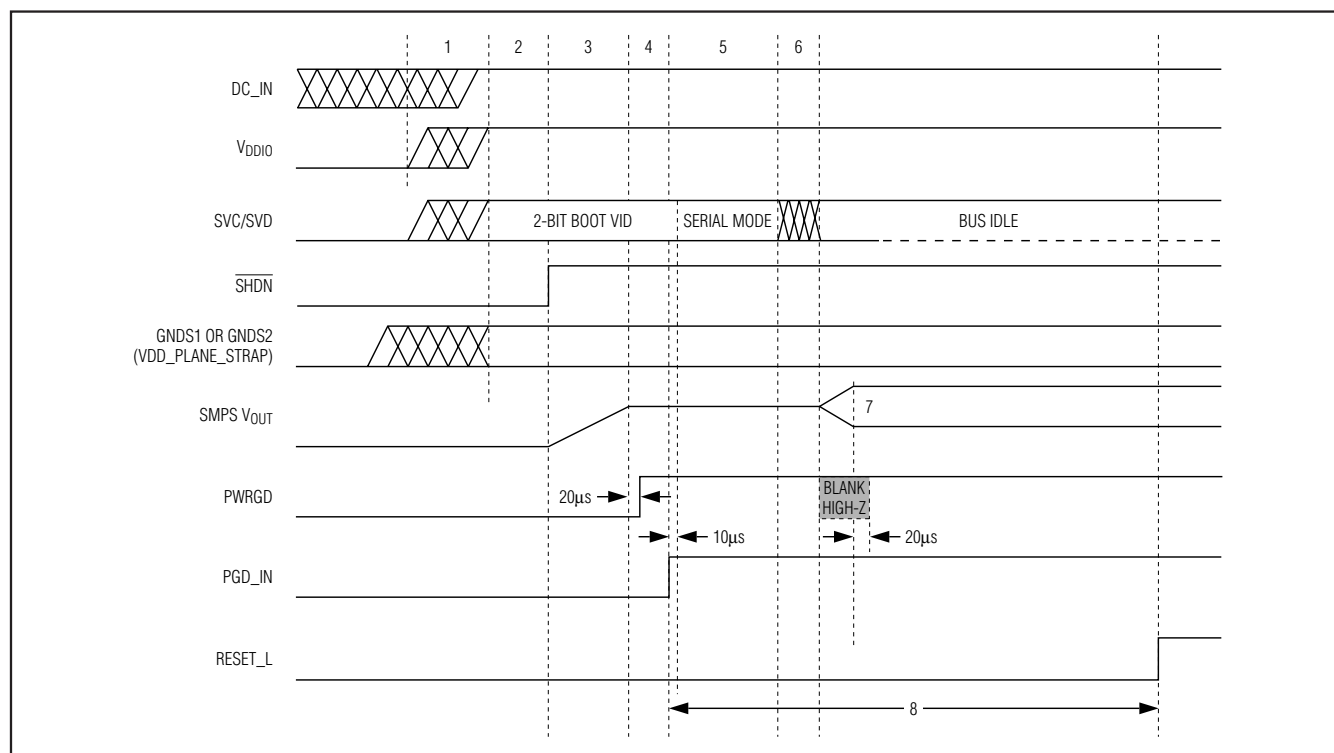
Figure 7. Startup Sequence
