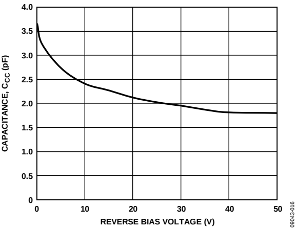
Figure 16. Collector-to-Collector Capacitance vs. Reverse Bias Voltage
