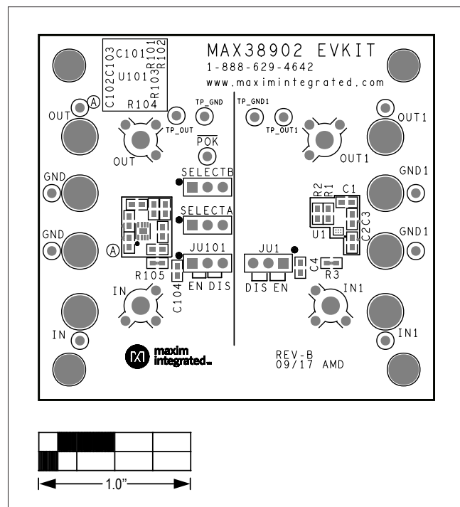
MAX38902 EV Kit—Top Silkscreen
