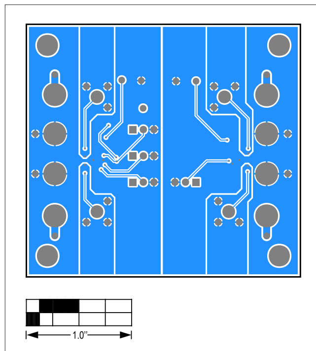
MAX38902 EV Kit—Bottom View
