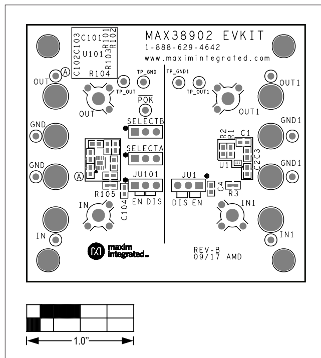
MAX38902 EV Kit—Bottom Silkscreen
