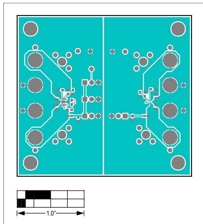
MAX38902 EV Kit—Top View
