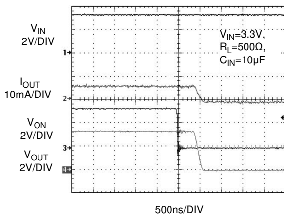
Figure 15. T_{OFF} Response
