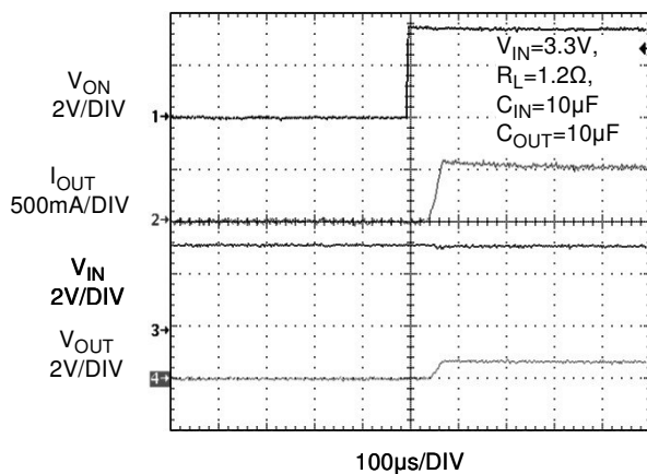
Figure 17. Current Limit Response (Output is loaded with 1.2Ω resistor and C_{OUT}=10\mu F )
