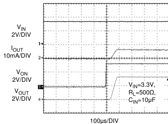
Figure 14. T_{ON} Response
