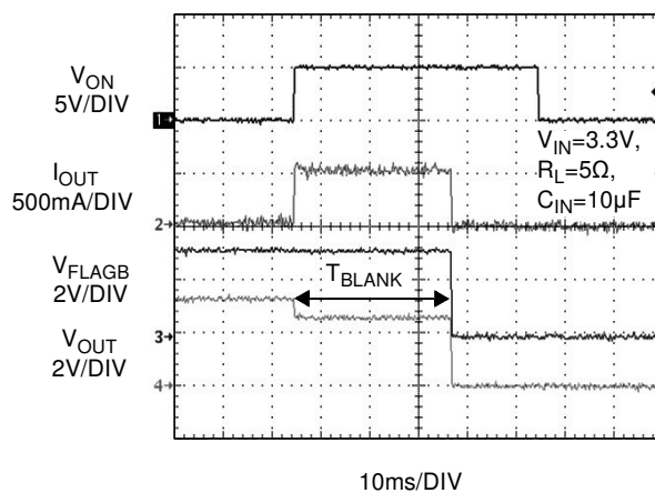
Figure 16. T_{BLANK} Response
