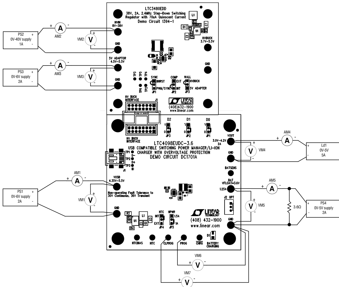
Figure 1. Proper Measurement Equipment Setup for DC1701A
