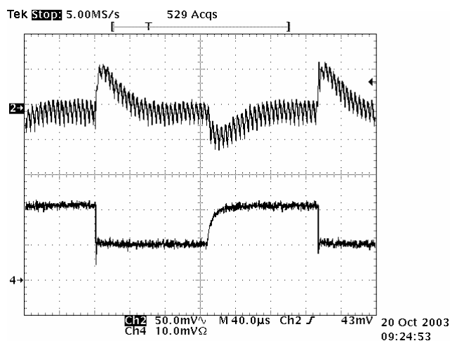
Figure 5. DC481 Typical Step Load Response ( I_{OUT} = 500\text{mA} to 1\text{A} , V_{IN} = 42\text{V} , T_A = 25^\circ\text{C} , V_{OUT} = 3.3\text{V} ) CH2 is V_{OUT} (AC) CH4 is I_{OUT} (500mA/10mVΩ)
