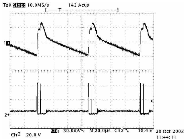
Figure 10. DC481 Typical Output Voltage Ripple in Burst Mode ( I_{OUT} = 100mA , V_{IN} = 42V , V_{OUT} = 3.3V , T_A = 25^\circ C ) CH1 is V_{OUT} ripple (AC), CH2 is V_{SW}
