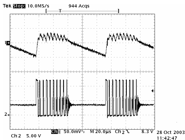
Figure 9. DC481 Typical Output Voltage Ripple in Burst Mode ( I_{OUT} = 100mA , V_{IN} = 12V , V_{OUT} = 3.3V , T_A = 25^\circ C ) CH1 is V_{OUT} ripple (AC), CH2 is V_{SW}
