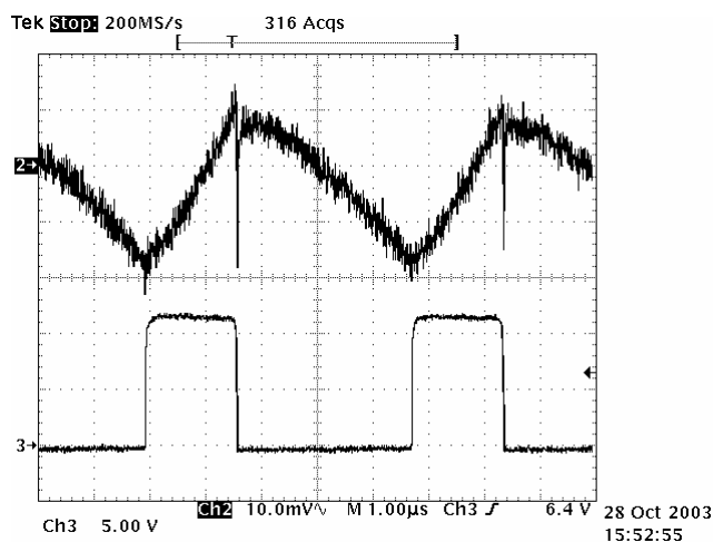
Figure 7. DC481 Typical Output Voltage Ripple ( I_{OUT} = 1\text{A} , V_{IN} = 12\text{V} , V_{OUT} = 3.3\text{V} , T_A = 25^\circ\text{C} ) CH2 is V_{OUT} ripple (AC), CH3 is V_{SW}
