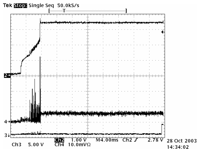
Figure 12. DC481 Soft Startup ( R_{LOAD} = 7\Omega , V_{IN} = 42V , V_{OUT} = 3.3V , T_A = 25^\circ C ) CH2 is V_{OUT} , CH3 is Power Good, CH4 is I_{IN} (100mA/10.0mVΩ)
