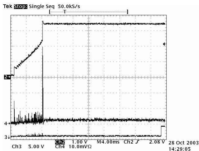
Figure 11. DC481 Soft Startup ( R_{LOAD} = 3.3\Omega , V_{IN} = 12V , V_{OUT} = 3.3V , T_A = 25^\circ C ) CH2 is V_{OUT} , CH3 is Power Good, CH4 is I_{IN} (200mA/10.0mVΩ)
