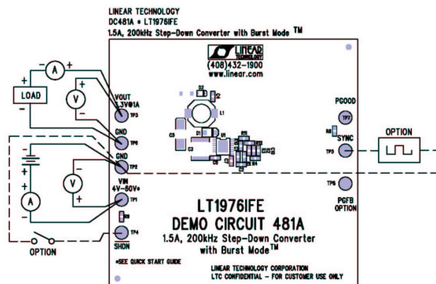
Figure 1. Proper Measurement Equipment Setup
