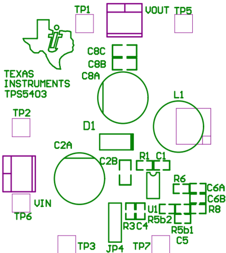
Figure 1. Placement (Top Layer)
