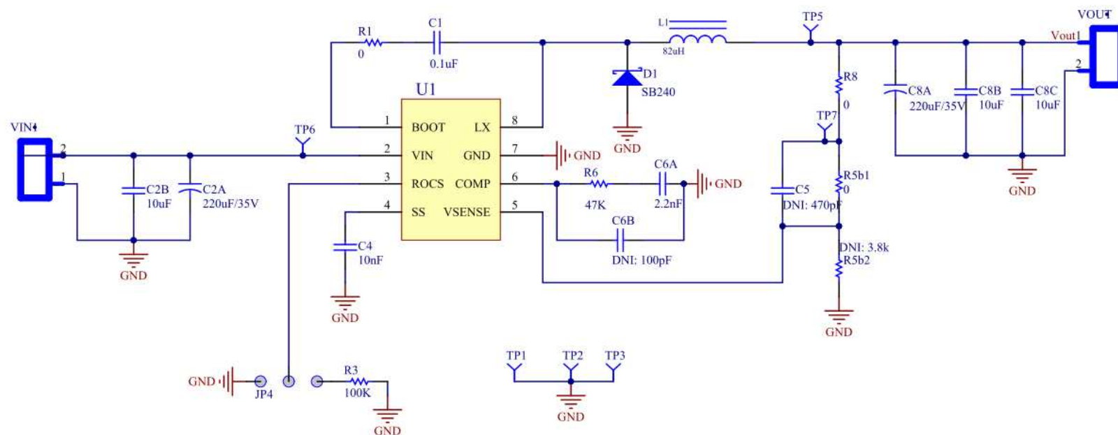
Figure 5. TPS5403EVM Schematic
