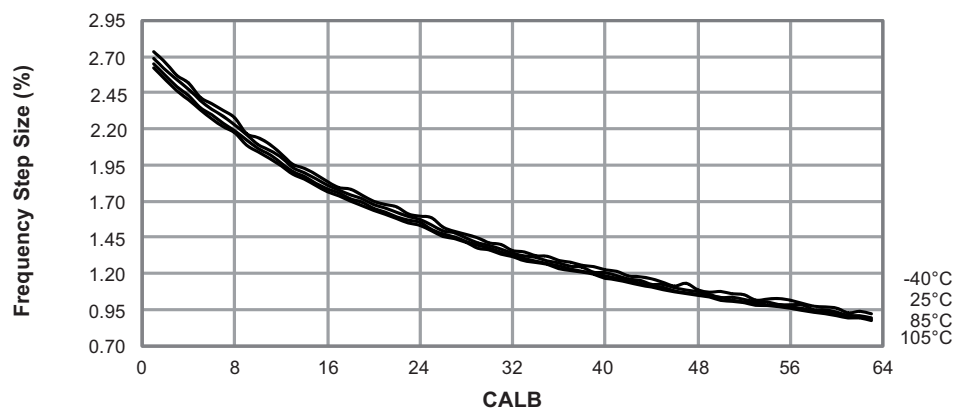
Figure 31-32. Internal 2MHz Oscillator CALB Calibration Step Size
