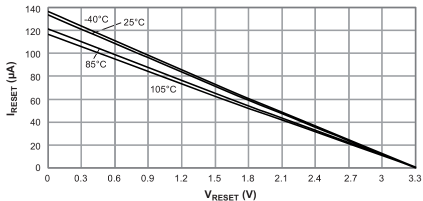
Figure 31-19. Reset Pull-up Resistor Current versus Reset Pin Voltage V_{CC} = 3.3V
