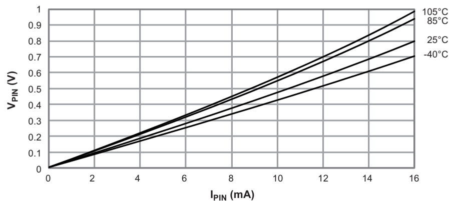
Figure 31-22. I/O Pin Output Voltage versus Sink Current V_{CC} = 3.0V
