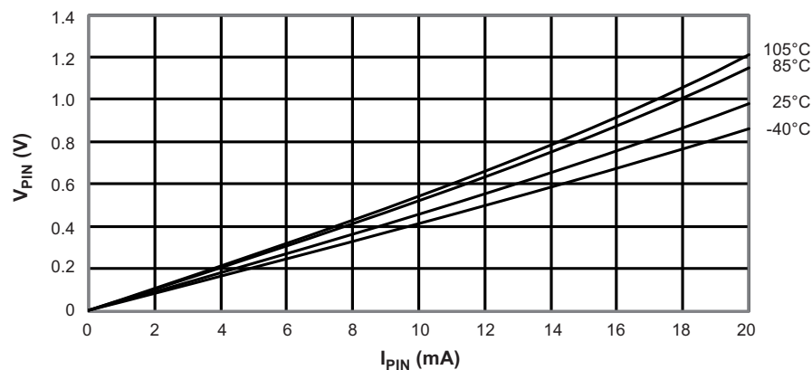
Figure 31-23. I/O Pin Output Voltage versus Sink Current V_{CC} = 3.3V
