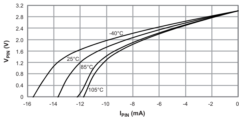
Figure 31-20. I/O Pin Output Voltage versus Source Current V_{CC} = 3.0V
