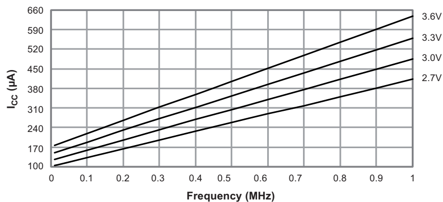
Figure 31-1. Active Supply Current versus Frequency f_{\text{SYS}} = 0 - 1\text{MHz} External Clock, T = 25^\circ\text{C}
