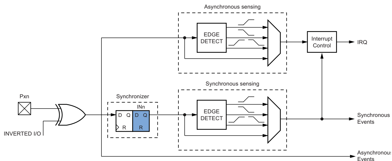
Figure 13-7. Input Sensing System Overview
