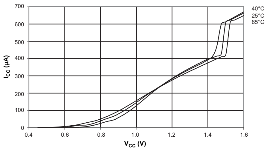
Figure 31-35. Power-up Current Consumption versus V_{CC}
