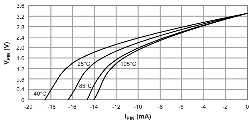
Figure 31-21. I/O Pin Output Voltage versus Source Current V_{CC} = 3.3V
