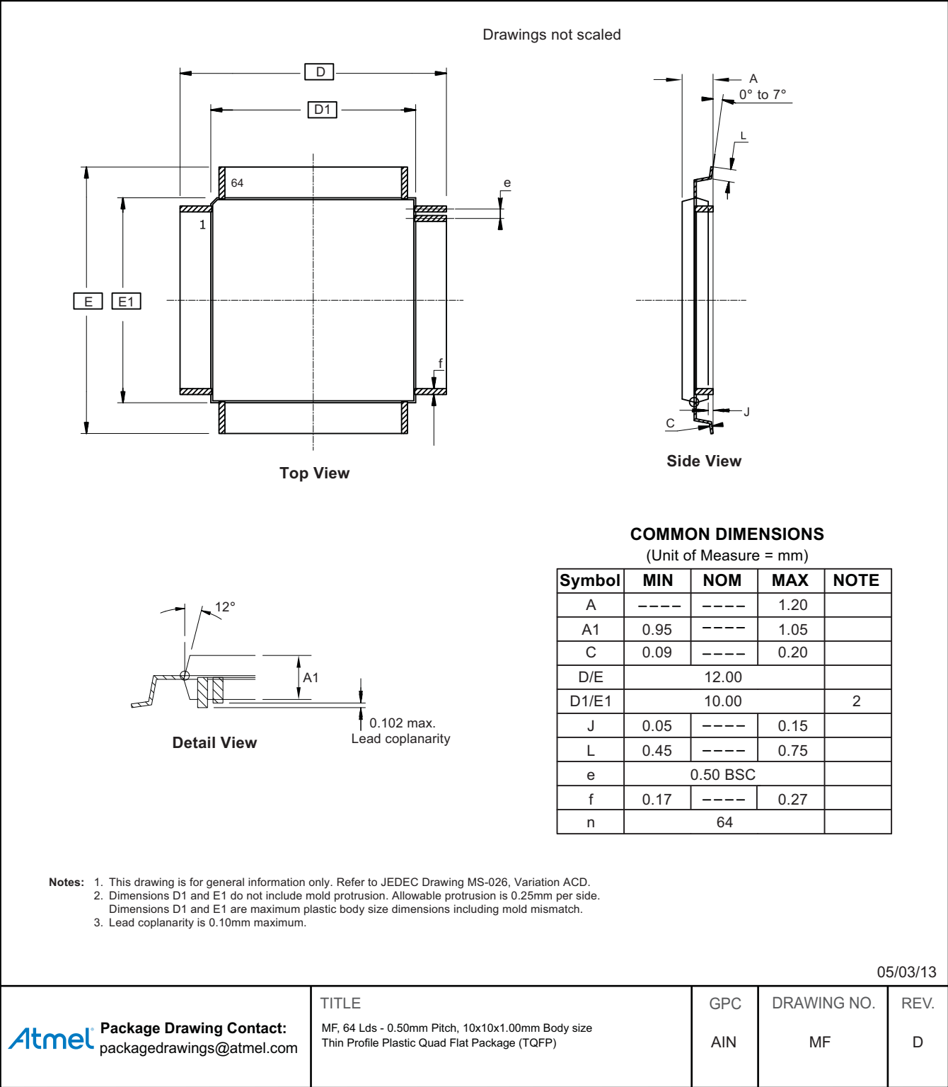
Figure 34-2. Package MF
