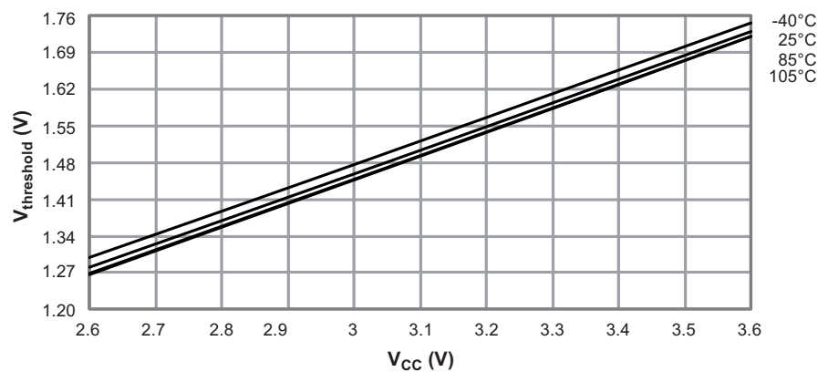
Figure 31-24. I/O Pin Input Threshold Voltage versus V_{CC} V_{IH} - Pin Read as "1"
