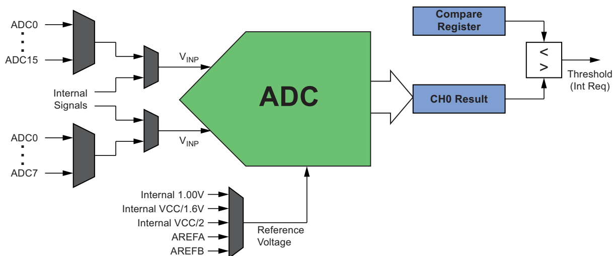
Figure 24-1. ADC Overview
