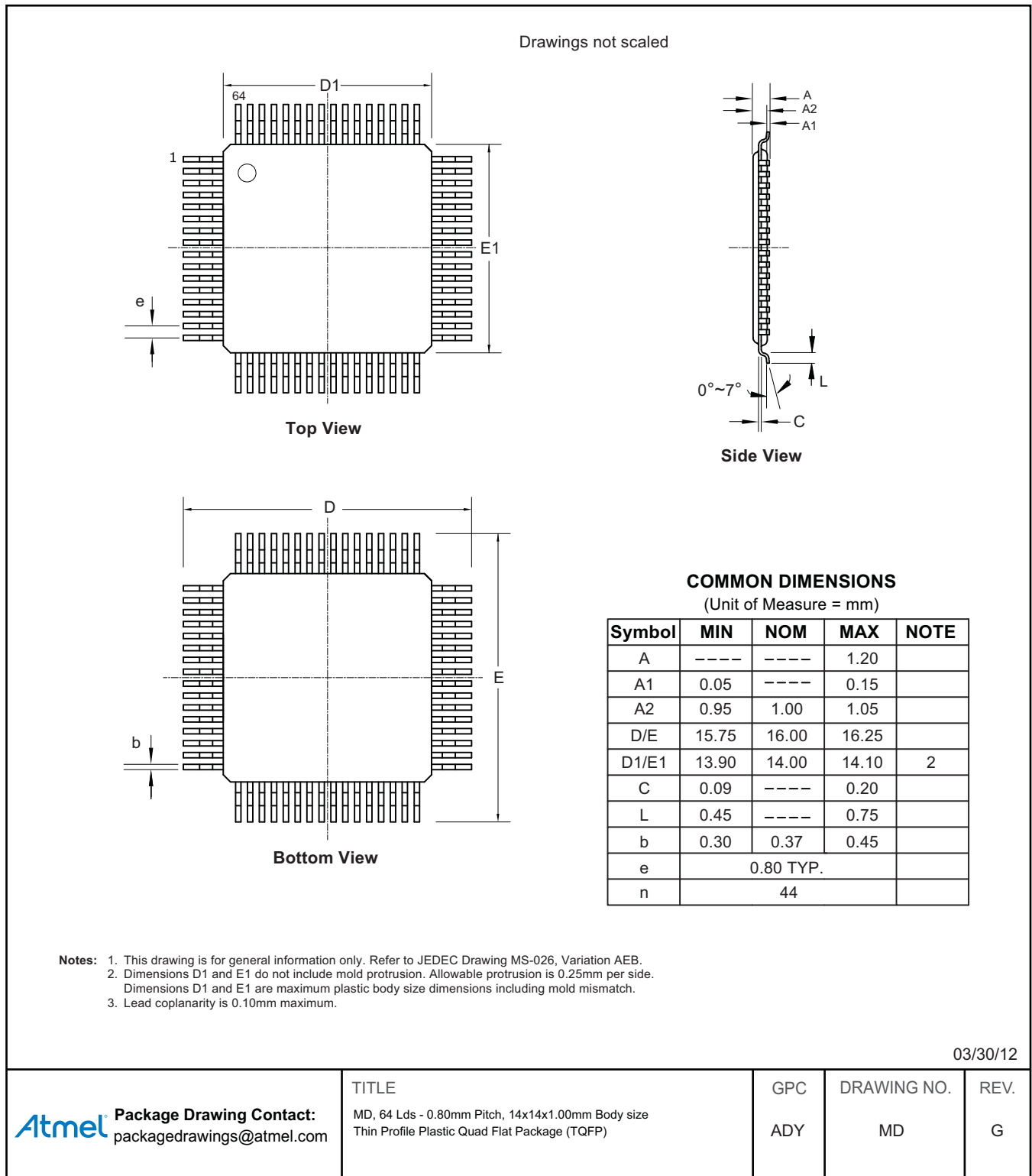
Figure 34-1. Package MD
