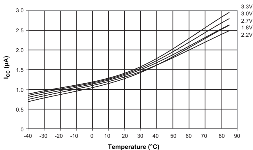
Figure 31-17. Power-save Supply Current versus Temperature with WDT, Sampled BOD, and RTC from ULP Enabled
