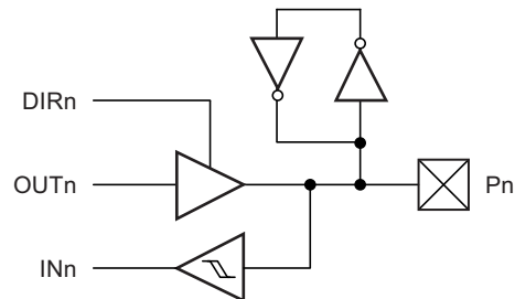
Figure 13-4. I/O Configuration - Totem-pole with Bus-keeper
