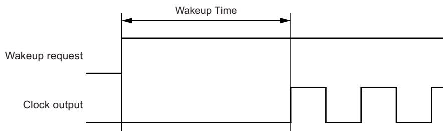
Figure 30-2. Wake-up Time Definition
