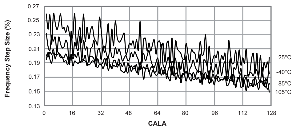
Figure 31-33. Internal 32MHz Oscillator CALA Calibration Step Size,
