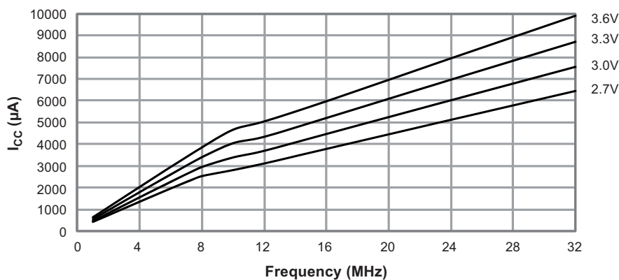
Figure 31-2. Active Supply Current versus Frequency f_{\text{SYS}} = 1 - 32\text{MHz} External Clock, T = 25^\circ\text{C}
