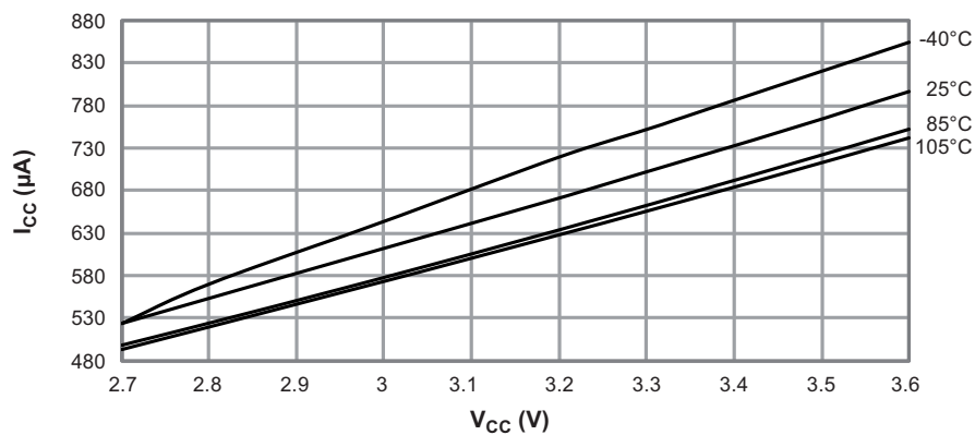
Figure 31-3. Active Supply Current versus V_{\text{CC}} f_{\text{SYS}} = 1\text{MHz} External Clock
