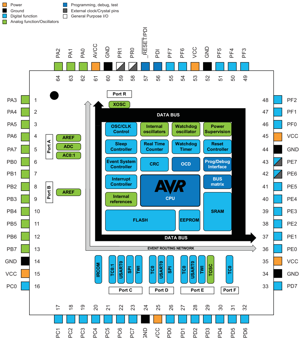
Figure 1-1. Block Diagram and Pinout
