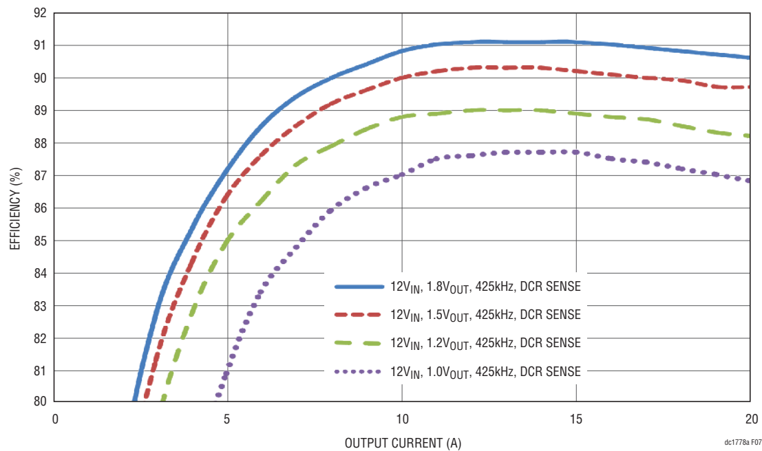
Figure 7. Typical Efficiency Curves, DC1778A-B DCR Current Sensing, 1.8V OUT , 12V IN , f SW = 425kHz
