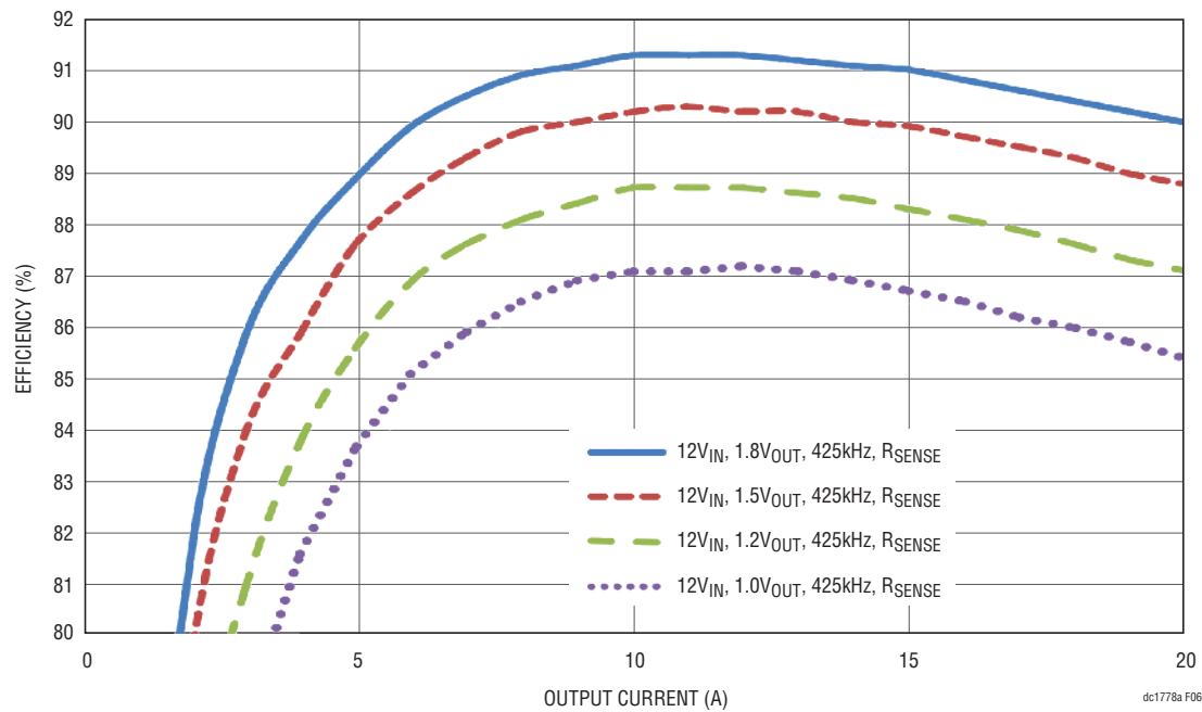
Figure 6. Typical Efficiency Curves, DC1778A-A Sense Resistor Current Sensing, 1.8V OUT , 12V IN , f SW = 425kHz
