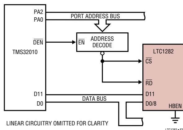
Figure 23. TMS32010 Interface
