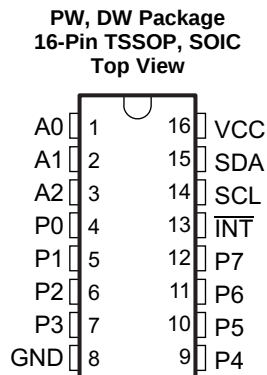
Pin Functions
