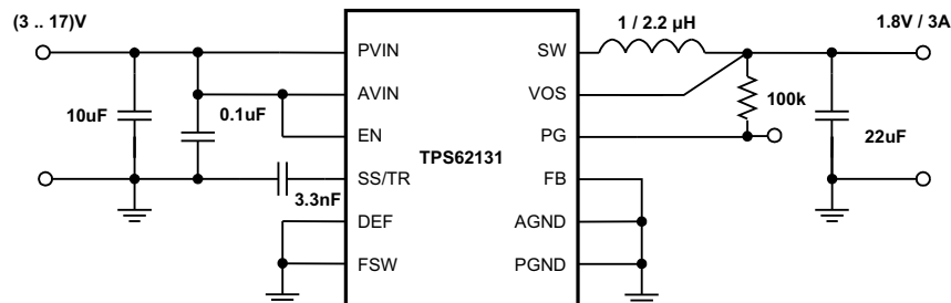
Figure 52. 1.8V/3A Power Supply
