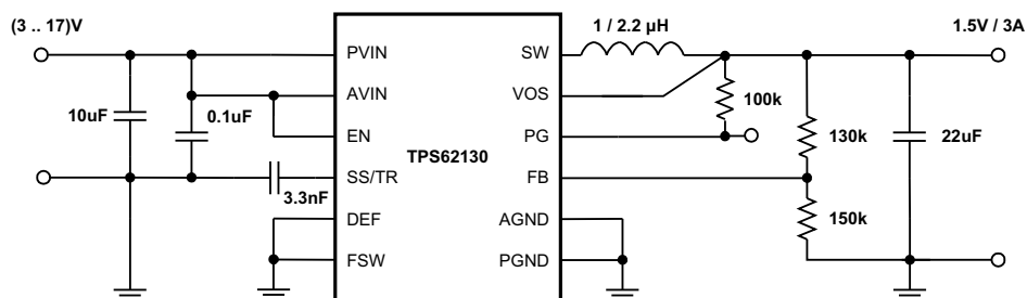
Figure 53. 1.5V/3A Power Supply
