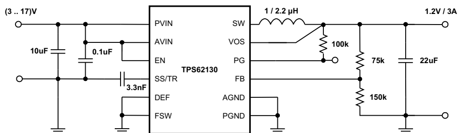
Figure 54. 1.2V/3A Power Supply
