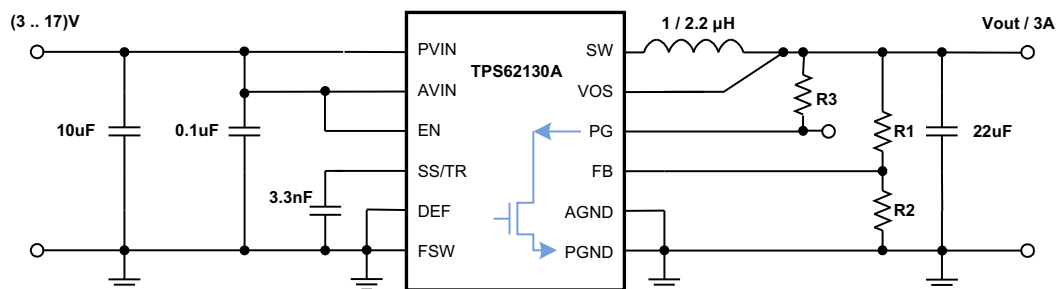
Figure 47. Discharge V OUT Through PG Pin with TPS62130A
