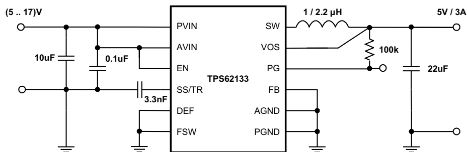
Figure 49. 5V/3A Power Supply
