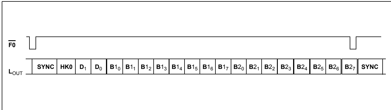
Figure 12 - Frame Format - 160 kbit/s (Modes 0, 2, 3, 4, 6)
