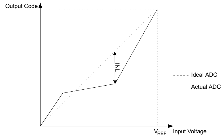
Figure 28-4. Integral Non-Linearity
