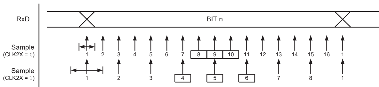
Figure 22-7. Sampling of Data and Parity Bits
