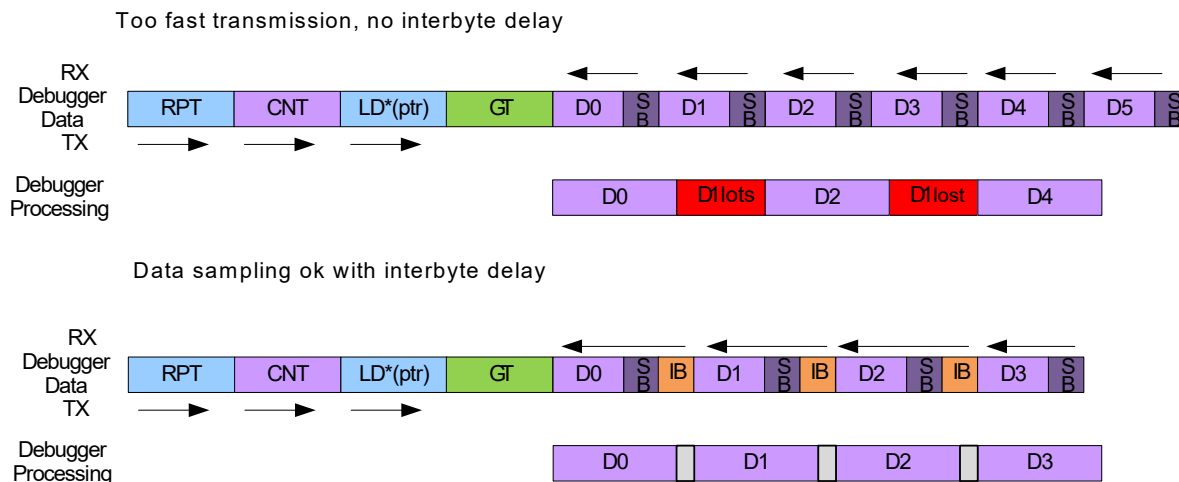
Figure 29-16. Interbyte Delay Example with LD and RPT
