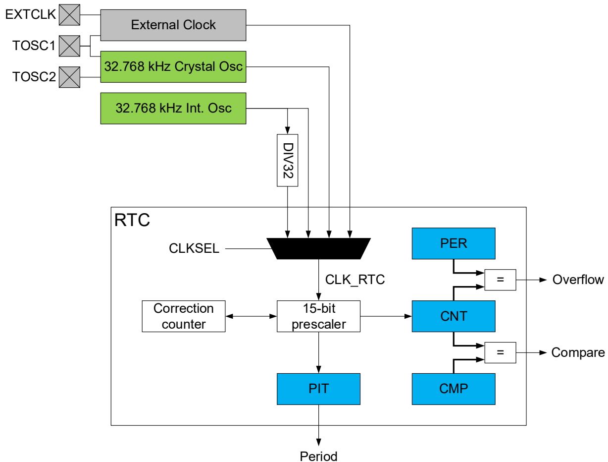
Figure 21-1. Block Diagram
