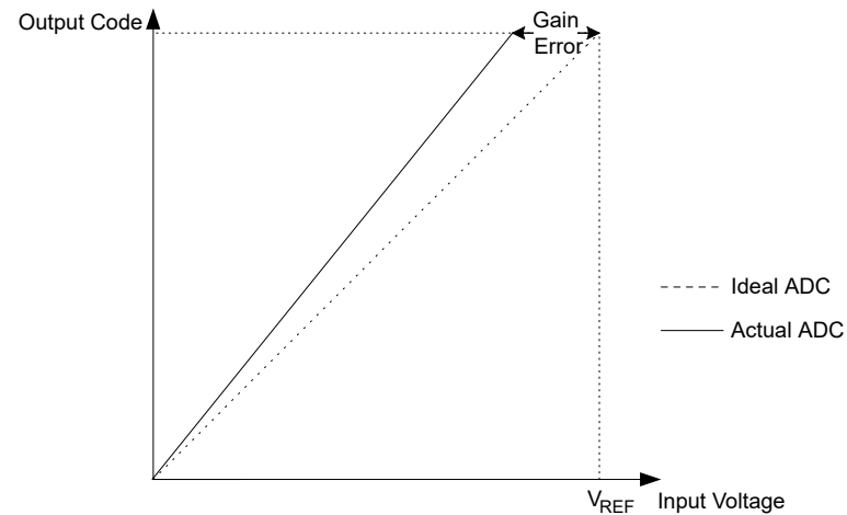
Figure 28-3. Gain Error
