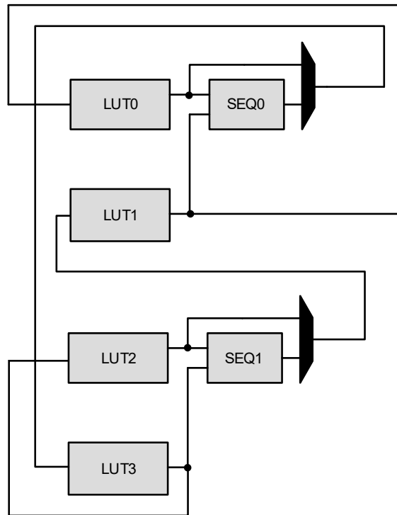
Figure 26-4. Linked LUT Input Selection
