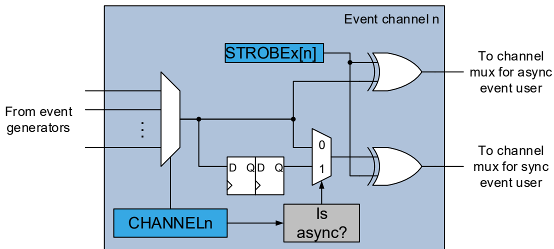
Figure 13-1. Block Diagram
