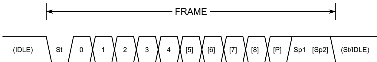
Figure 22-2. Frame Formats
