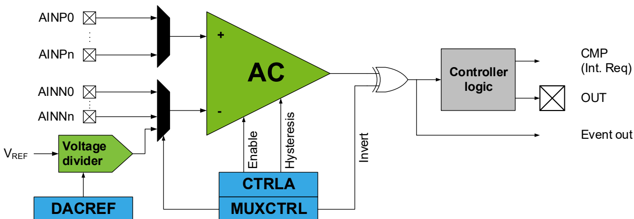
Figure 27-1. Analog Comparator
