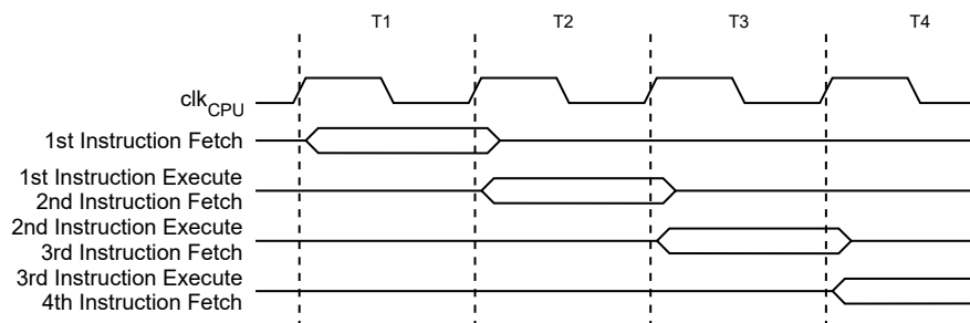
Figure 7-2. The Parallel Instruction Fetches and Executions
