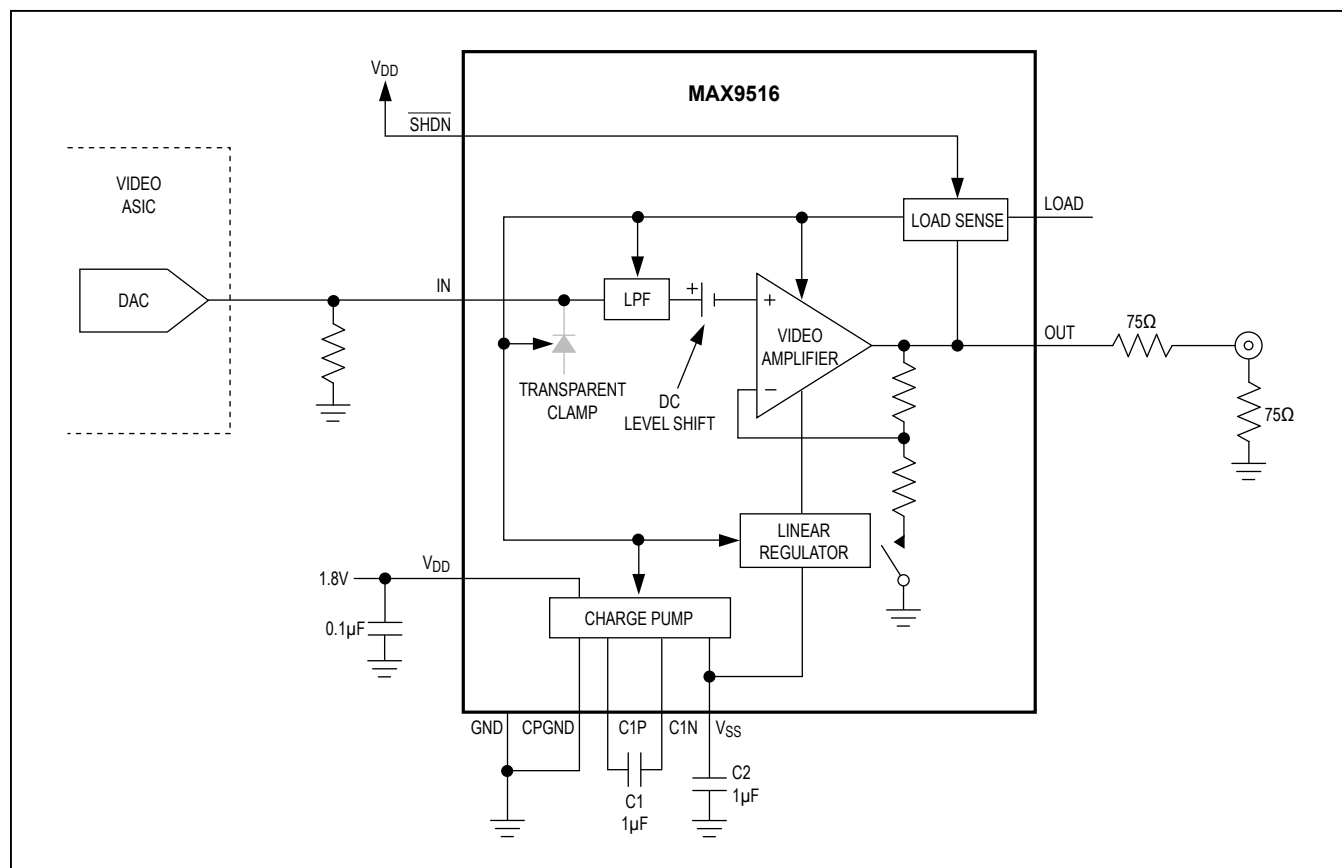
Figure 7. DC-Coupled Input
