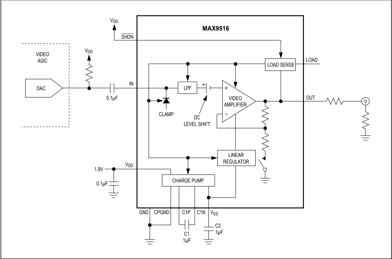
Figure 8. AC-Coupled Input
