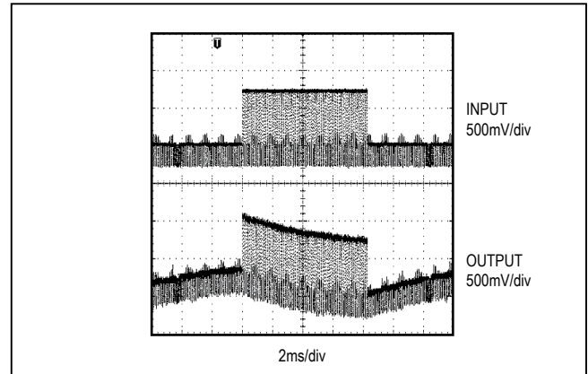
Figure 1. AC-Coupled Output
