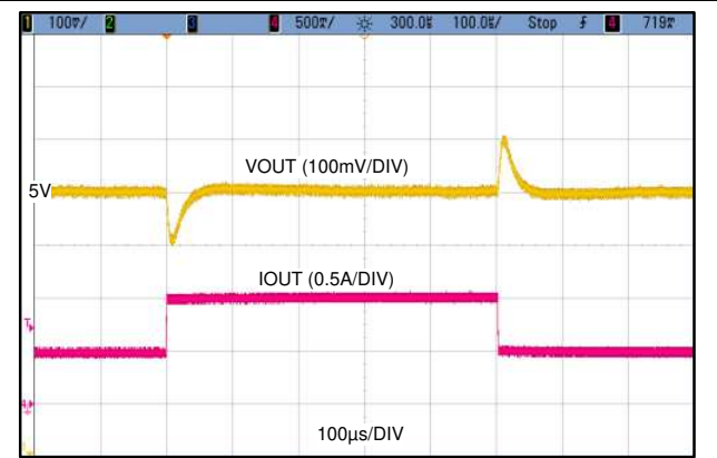
Figure 29. Load Transient
