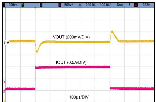
Figure 28. Load Transient
