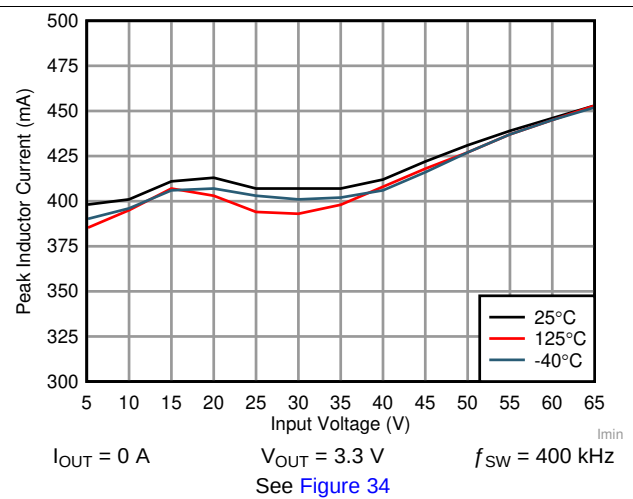
Figure 2. I_{PEAK-MIN}
