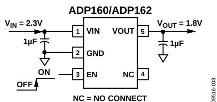
Figure 3. Typical ADP160/ADP162 Application Circuit
