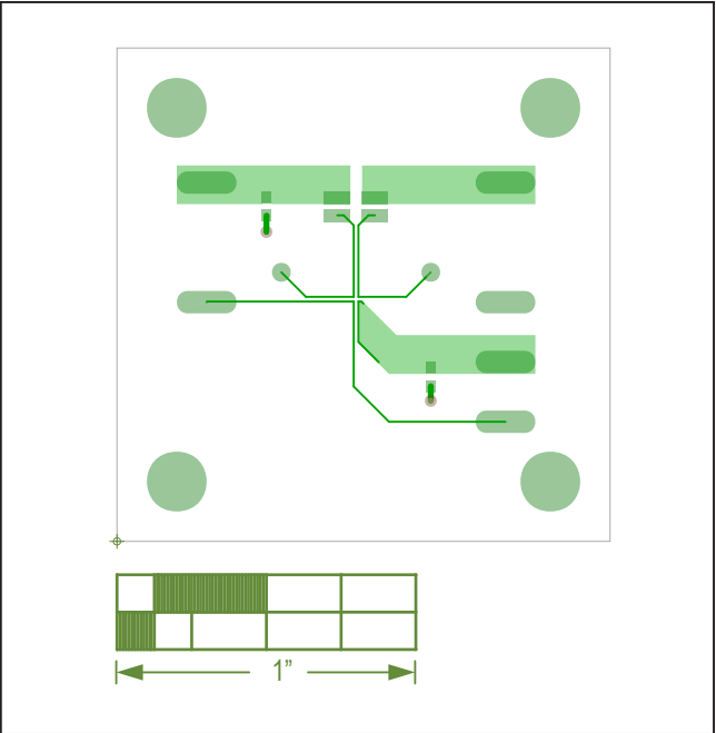
Figure 3. MAX44286 EV Kit PCB Layout—Component Side
