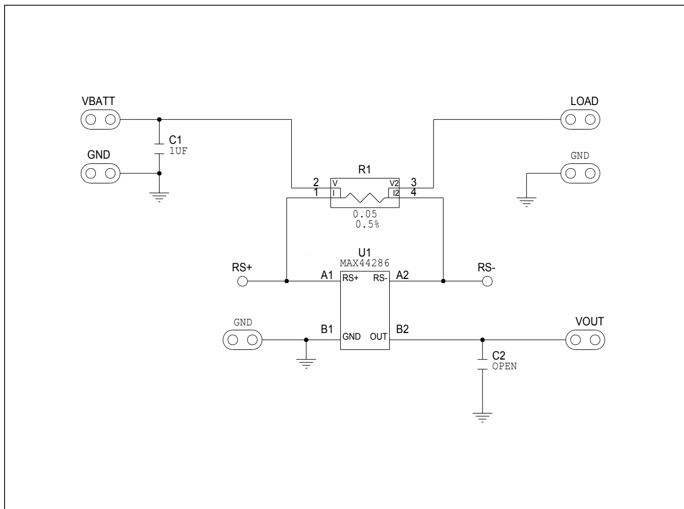
Figure 1. MAX44286 EV Kit Schematic
