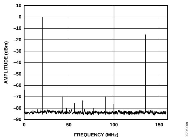
Figure 9. Single-Tone Spectrum @ f_{DATA} = 78\text{ MSPS} with f_{OUT} = f_{DATA}/3
