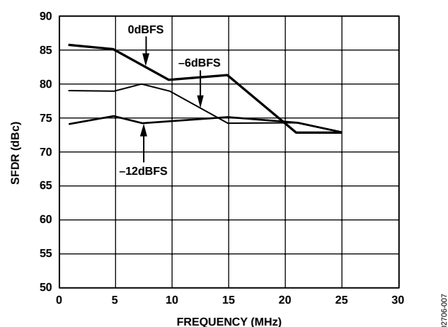
Figure 7. In-Band SFDR vs. f_{OUT} @ f_{DATA} = 65\text{ MSPS}
