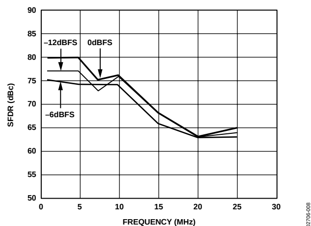
Figure 8. Out-of-Band SFDR vs. f_{OUT} @ f_{DATA} = 65\text{ MSPS}
