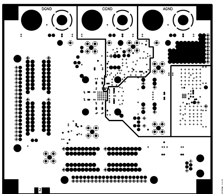
Figure 112. AD9777 Evaluation Board Layout, Layer Two (Ground Plane)
