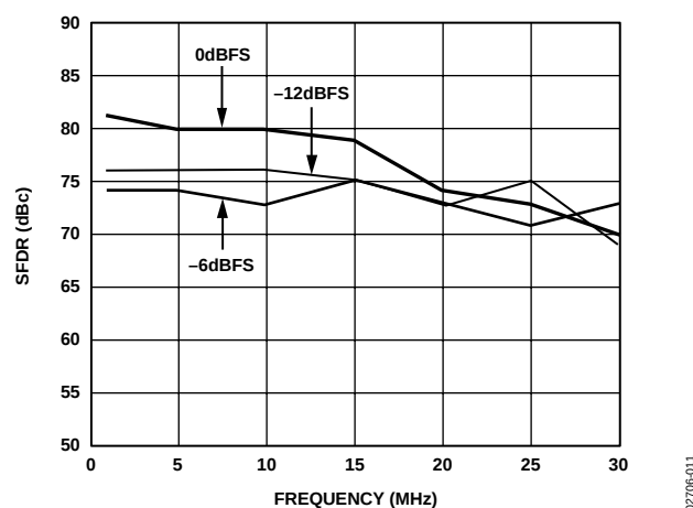
Figure 11. Out-of-Band SFDR vs. f_{OUT} @ f_{DATA} = 78\text{ MSPS}
