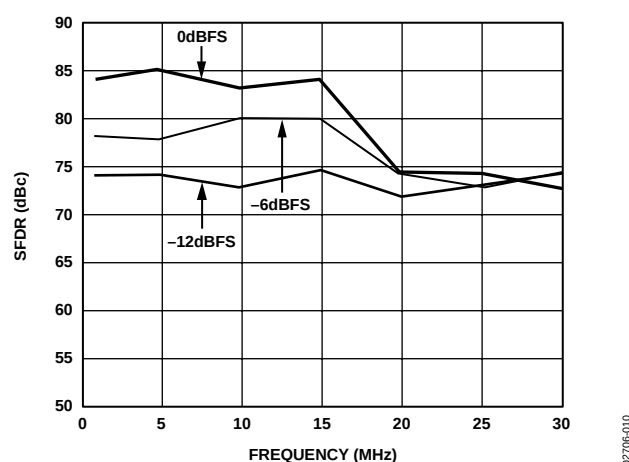
Figure 10. In-Band SFDR vs. f_{OUT} @ f_{DATA} = 78\text{ MSPS}
