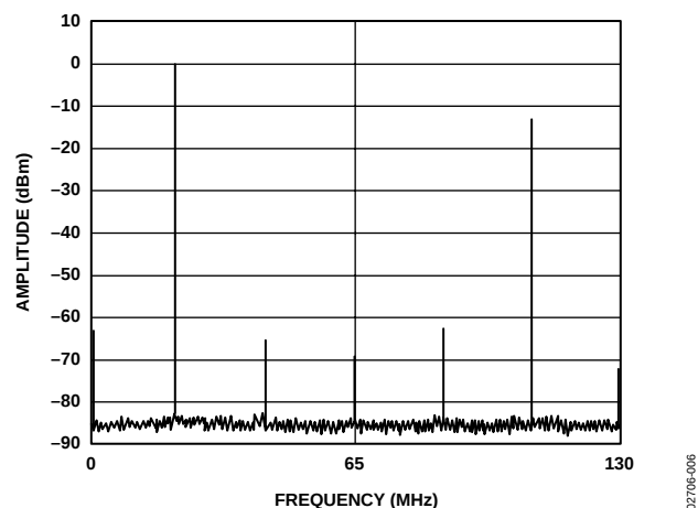
Figure 6. Single-Tone Spectrum @ f_{DATA} = 65\text{ MSPS} with f_{OUT} = f_{DATA}/3
