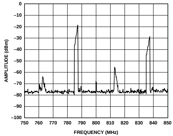
Figure 94. AD9777 Complex Output from Figure 93, Now Quadrature Modulated by AD8345 (LO = 800 MHz)
