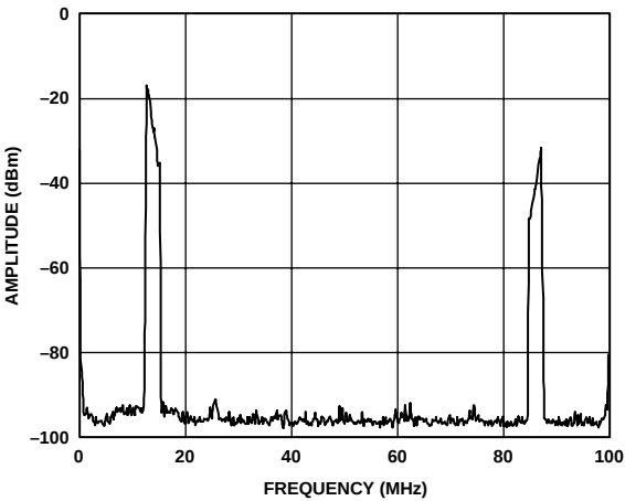
Figure 95. AD9777, Real DAC Output of Complex Input Signal Near Baseband (Positive Frequencies Only), Interpolation = 8 \times , Complex Modulation in AD9777 = +f_{DAC}/8
