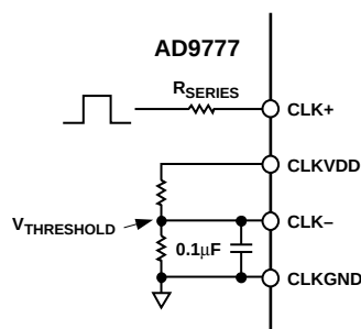
Figure 43. Single-Ended Clock Driving Clock Inputs
