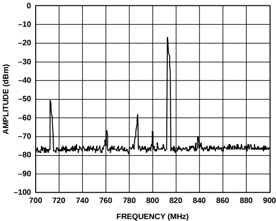
Figure 96. AD9777 Complex Output from Figure 95, Now Quadrature Modulated by AD8345 (LO = 800 MHz)
