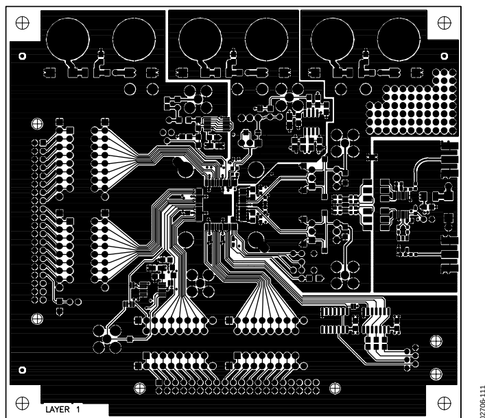
Figure 111. AD9777 Evaluation Board Layout, Layer One (Top)
