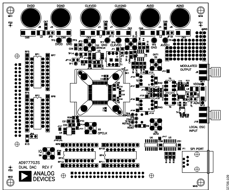
Figure 109. AD9777 Evaluation Board Components, Top Side
