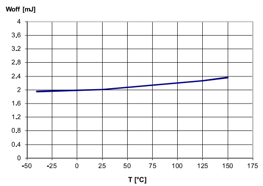
Figure 22: Woff vs. Tcase
