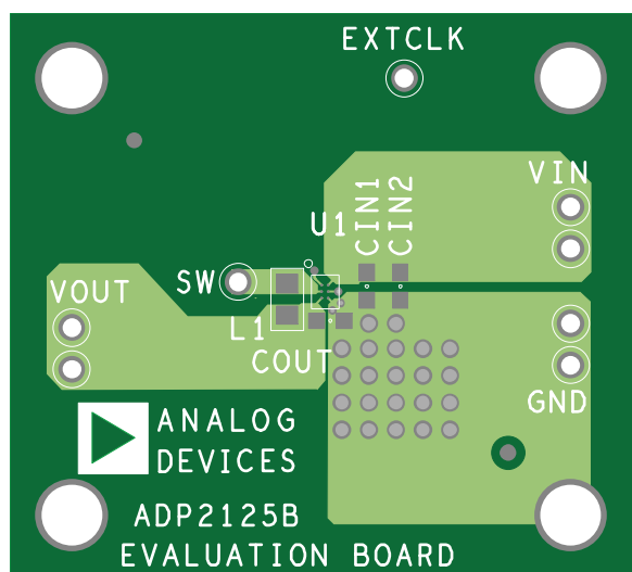
Figure 3. ADP2125 Top Layer
