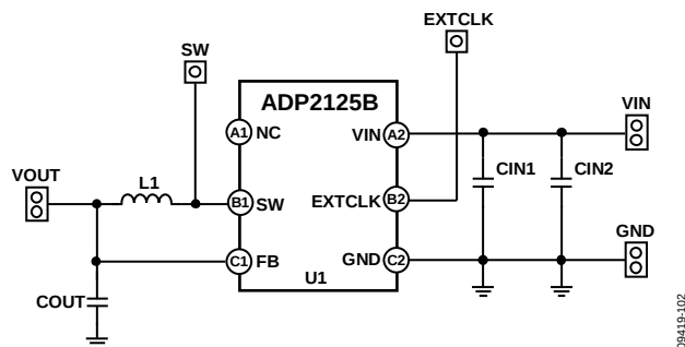
Figure 2. ADP2125 Evaluation Board Schematic
