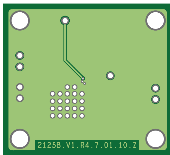
Figure 4. ADP2125 Bottom Layer
