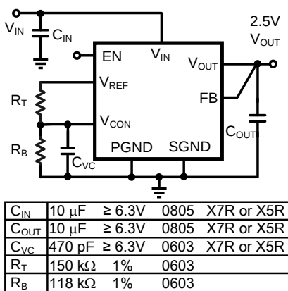
Figure 6. V_{OUT} = 2.5 V
