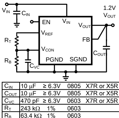
Figure 5. V_{OUT} = 1.2 V
