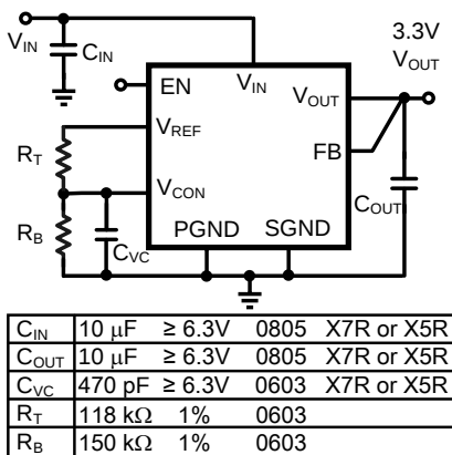
Figure 7. V_{OUT} = 3.3 V
