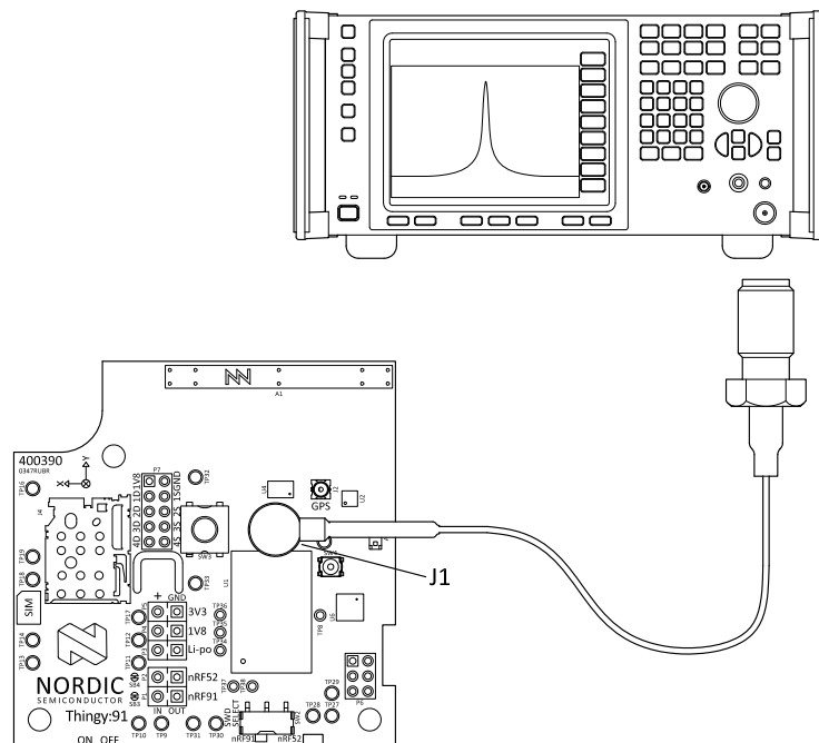
Figure 7: Connecting a spectrum analyzer
