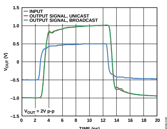
Figure 18. ADV3229 Large Signal Pulse Response
