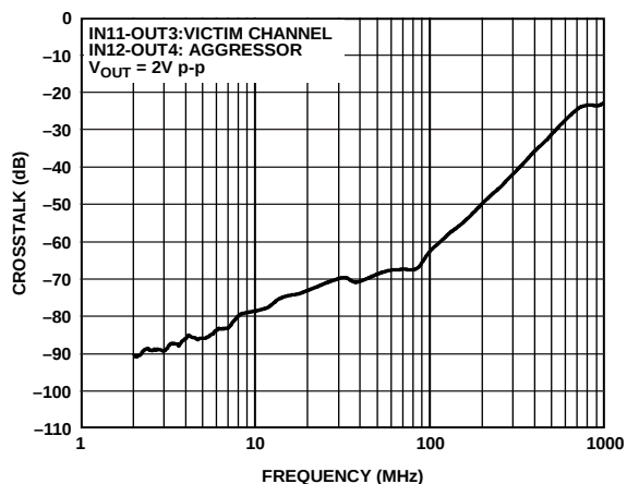
Figure 34. ADV3229 Crosstalk, One Adjacent Channel, RTO
