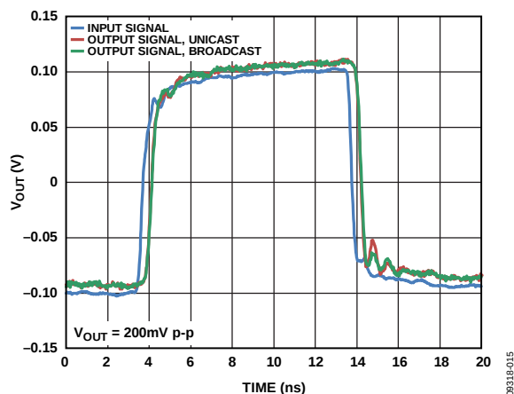
Figure 14. ADV3228 Small Signal Pulse Response
