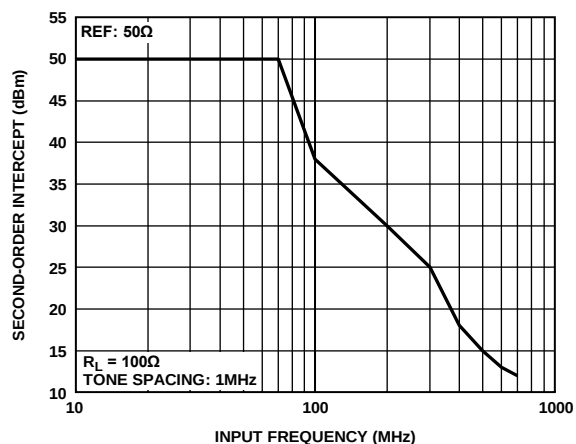
Figure 55. ADV3229 Second-Order Intercept, 100 \Omega Load
