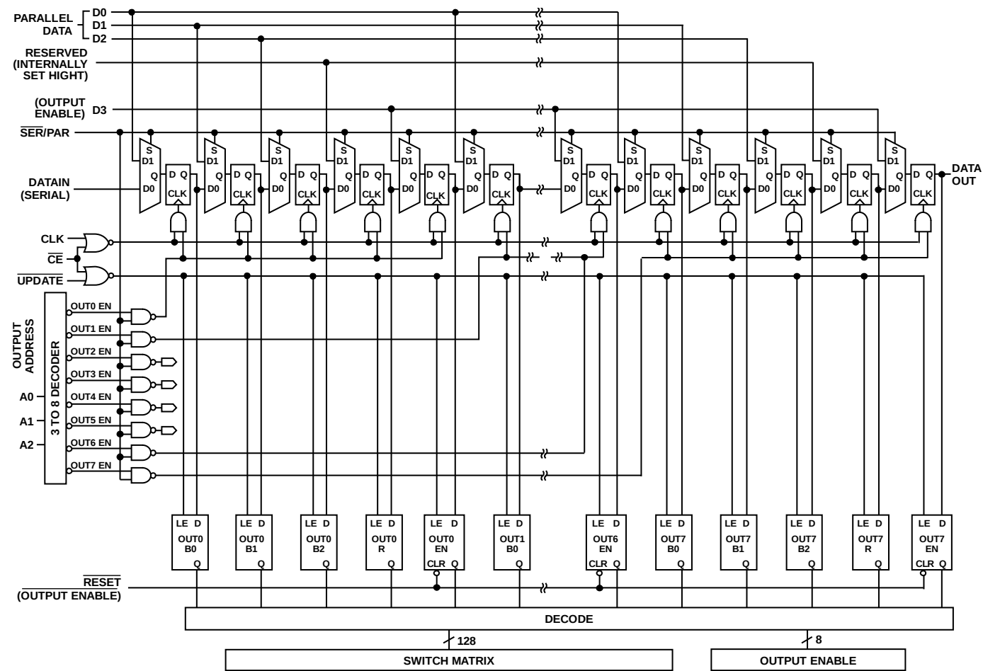
Figure 6. Logic Diagram
