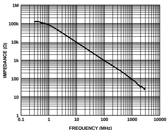
Figure 36. ADV3229 Input Impedance
