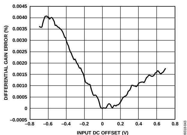
Figure 45. ADV3228 Differential Gain Error
