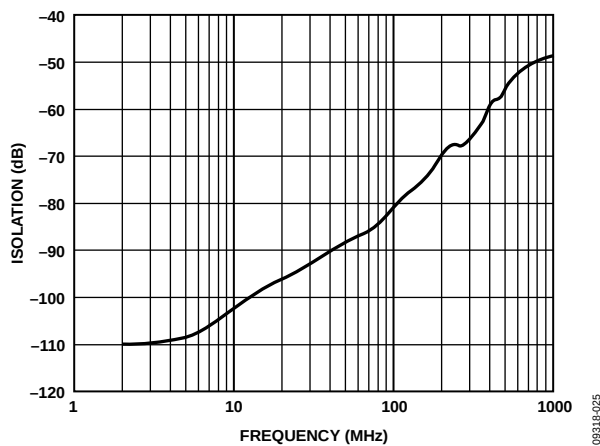
Figure 27. ADV3228 Off Isolation
