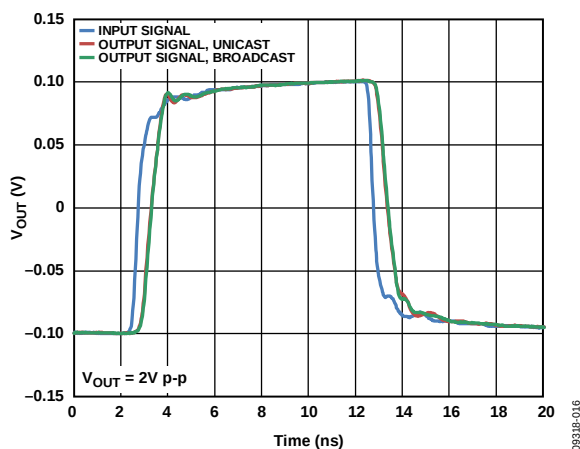
Figure 15. ADV3228 Large Signal Pulse Response
