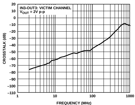
Figure 35. ADV3229 Crosstalk, All Hostile, RTO
