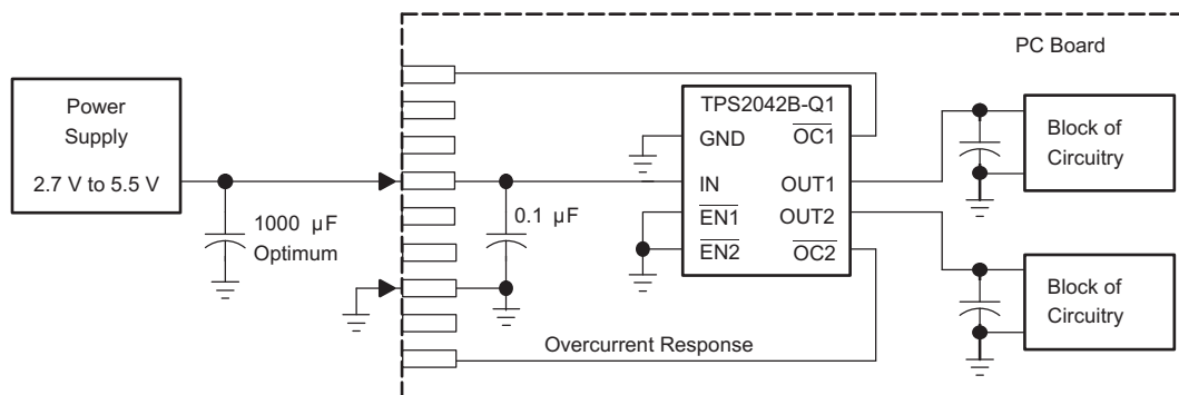
Figure 31. Example Hot-Plug Implementation (TPS2042B-Q1)
