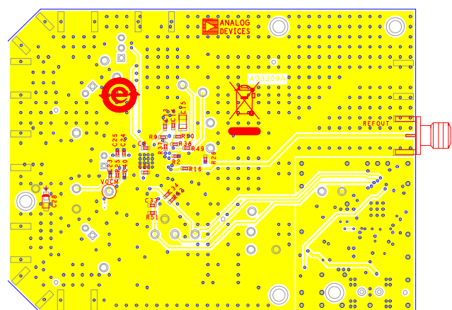
Figure 47. ADRF6807 Evaluation Board Bottom Layer
