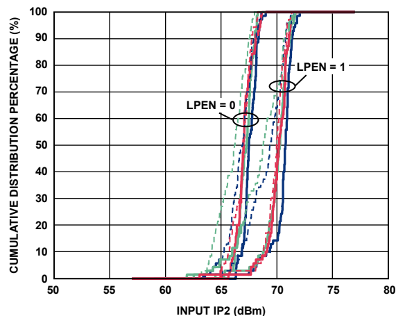
Figure 30. Input IP2
