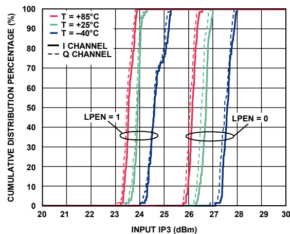
Figure 28. Input IP3
