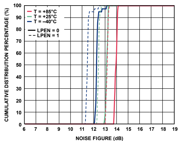
Figure 31. Noise Figure
