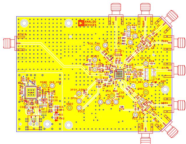
Figure 46. ADRF6807 Evaluation Board Top Layer
