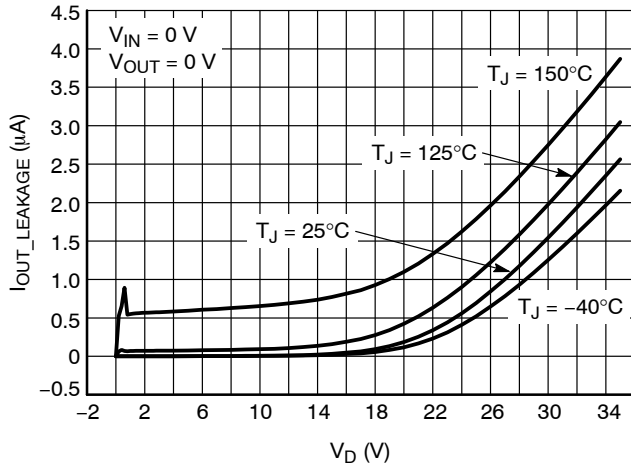
Figure 16. Output Leakage Current vs. V_D Voltage & Temperature, V_{OUT} = 0\text{ V}
