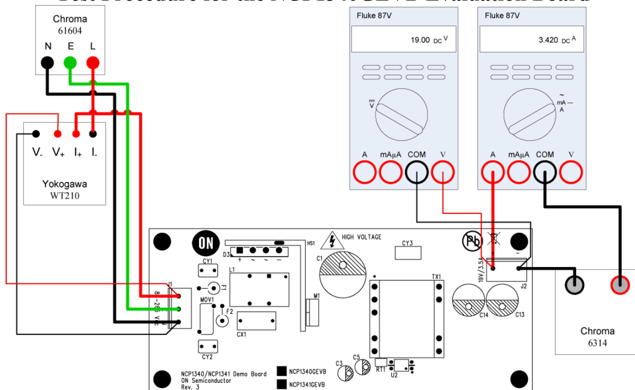
Figure 1: Test Setup
