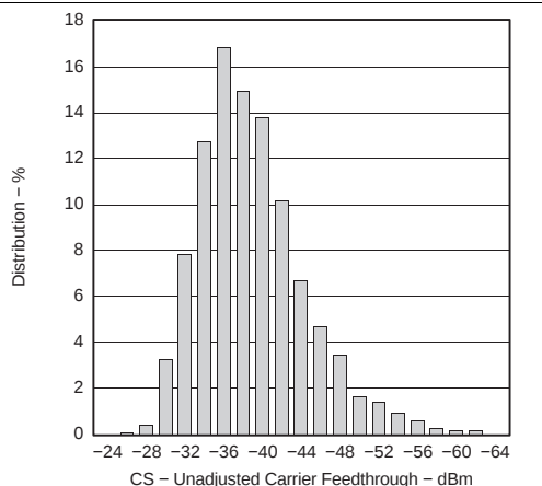
Figure 41. Unadjusted Carrier Feedthrough at 1600 MHz Distribution
