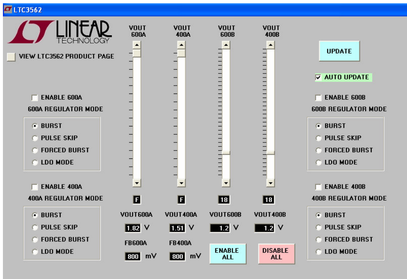
Figure 3. Graphical User Interface
