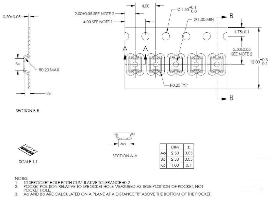
Figure 20. LGA-12 package orientation in carrier tape
