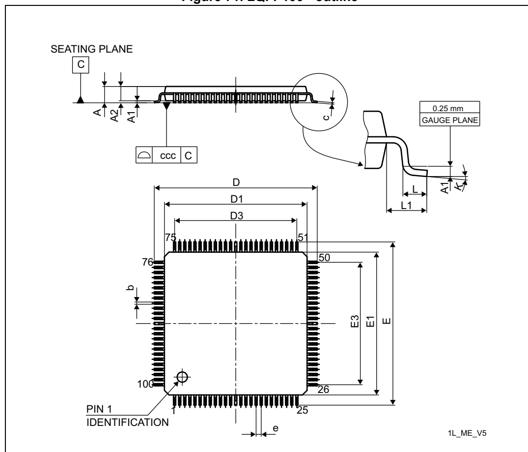
Figure 71. LQFP100 - outline
