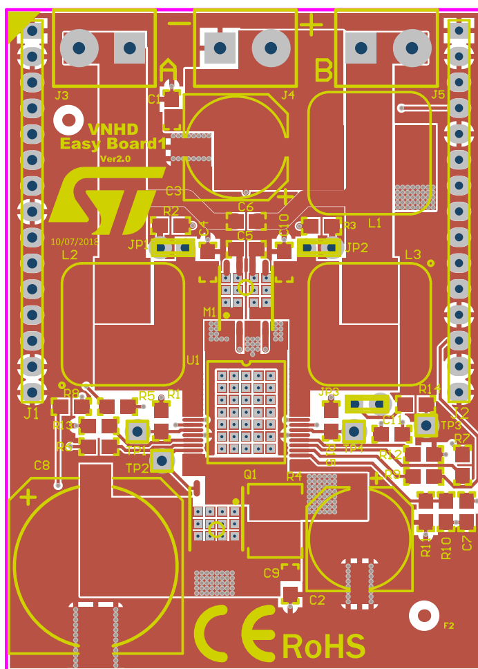
Figure 2. VNHD7008AY evaluation board top layout
