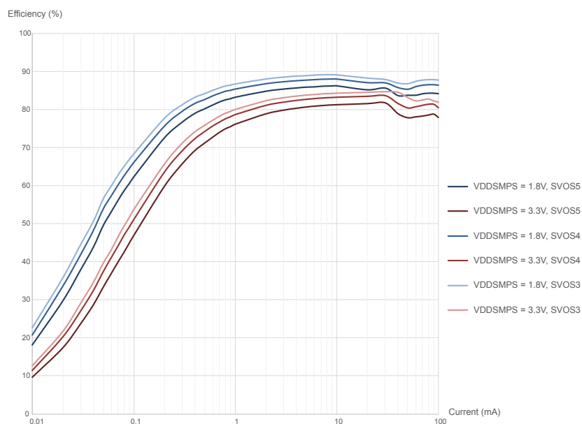
Figure 27. SMPS efficiency vs load current in Stop and DStop modes (SVOS3 LP mode, SVOS4, SVOS5), T_J = 130\text{ °C}
