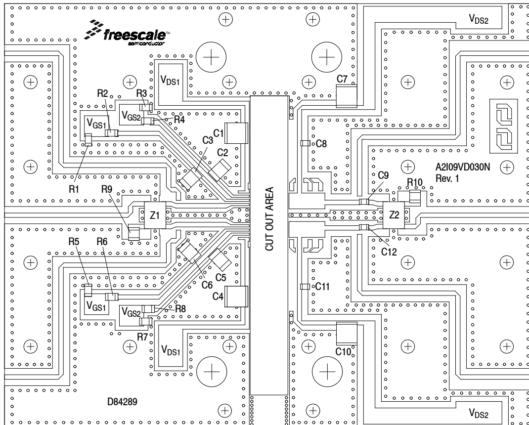
Figure 3. A2I09VD030NR1 Test Circuit Component Layout – 920-960 MHz
