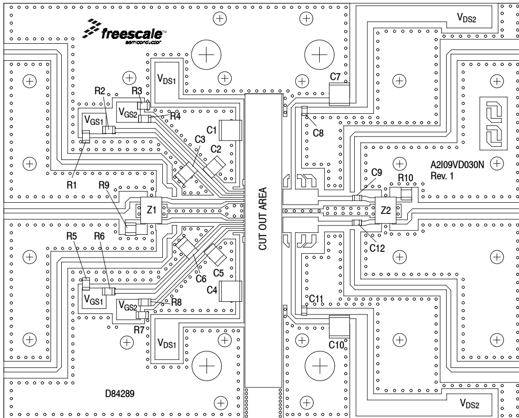
Figure 17. A2I09VD030NR1 Test Circuit Component Layout – 728-768 MHz
