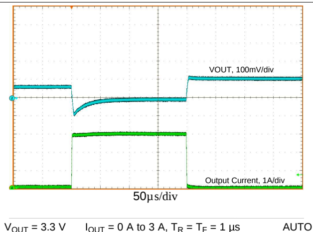
Figure 42. Load Transient
