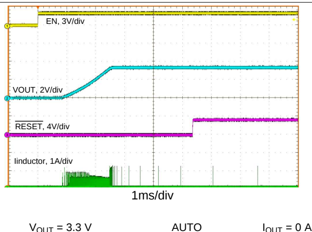
Figure 41. Start-up
