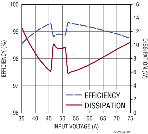
Figure 1. Efficiency and Dissipation at 18A Load
